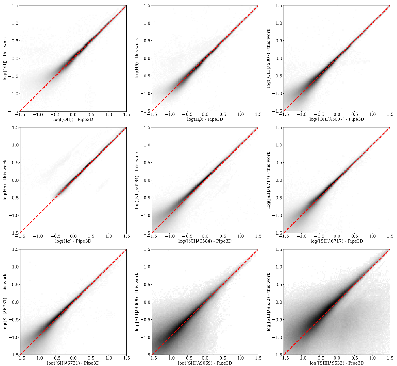
Fig. A.1. Spaxel-by-spaxel comparison between the emission line fluxes taken into account in this work (y-axis) and the results of Pipe3D (x-axis): namely [O II] \lambda 5007, H \beta , [O III] \lambda 5007, H \alpha , [N II] \lambda 6584, [S II] \lambda 6717, [S II] \lambda 6731, [S III] \lambda 9069, [S III] \lambda 9532. The fluxes are in units of 10^{-17} erg s ^{-1} \text{\AA}^{-1} cm ^{-2} and are expressed in logarithm. The red dashed line represents the one-to-one line.
