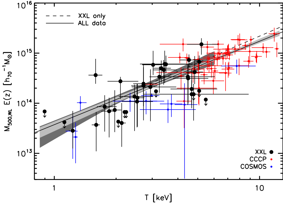
Fig. 5. Mass-temperature relation for the extended sample, including 38 systems from XXL (black), 10 from COSMOS (blue), and 48 from CCCP (red). The solid line and light grey shaded region are the best fit scaling relation and 68% credible interval for the XXL+COSMOS+CCCP sample. The dashed line and dark grey shaded region are the best fit and credible region for the XXL only sample. Systems with upper limits on mass are indicated by arrows and plotted at 3 sigma confidence.
