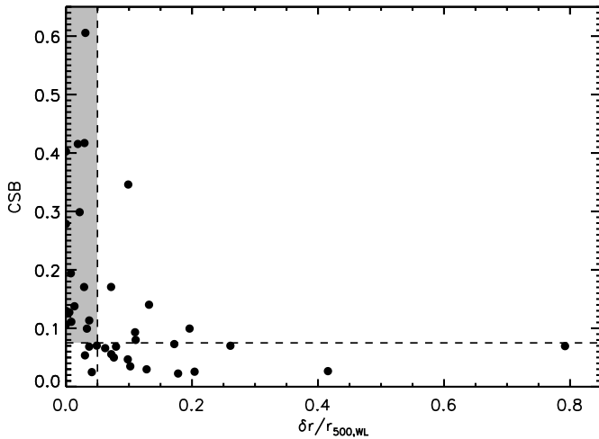
Fig. 6. CSB parameter versus the offset between X-ray centroid and BCG as a fraction of weak-lensing r_{500,WL} . The horizontal dashed line at CSB = 0.075 indicates the separation of cool core and non-cool core classed systems. The vertical dashed line at \delta r / r_{500,WL} = 0.05 separates undisturbed and disturbed clusters. The grey shaded region shows the overlap between cool core and undisturbed clusters.
