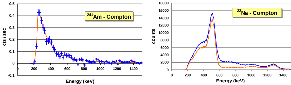
Figure 1. In the left panel, the background subtracted Compton spectrum obtained from an ^{241}\text{Am} acquisition (crosses), compared with the spectrum of random coincidences (continuous line) is shown. In the right panel the background subtracted ^{22}\text{Na} 'Compton single' spectra obtained before (upper curve) and after (lower curve) the subtraction of random coincidences is plotted.
