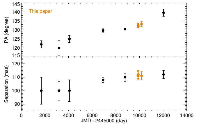
Fig. 6. Position in separation and position angle of the FUOR component relative to the HBe, based on the literature and our NaCo and Keck observations.
