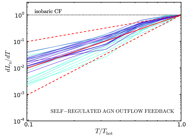
Figure 1. The X-ray spectrum in the form of differential luminosity distribution per temperature interval, for the reference self-regulated AGN outflow feedback model ( \epsilon \simeq 5 \times 10^{-3} ). As in observations (Section 1), we use the hot gas temperature in the core for the normalization ( T_{\text{hot}} \simeq 4 keV) and we extract the distribution within the cooling radius, r < 100 kpc ( \sim 1 arcmin for A1795). The distribution is normalized to the pure isobaric CF (dotted; equation 6). The colour coding is related to the accretion rates averaged over 20 Myr after each snapshot time (cyan to blue \approx 1 –20 M_\odot \text{ yr}^{-1} ). The simulated spectrum is consistent with the observational constraints (red; \alpha = 2 \pm 1 , equation 9), showing a strong deficit down to T \simeq 0.4 keV (we cut the plot to this value as it roughly corresponds to Chandra lower sensitivity). The departure from the standard isobaric CF naturally develops via the tight self-regulation between TI condensation and turbulent AGN heating.
