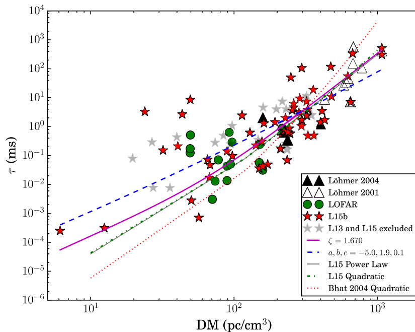
Figure 21. Scattering time ( \tau ) at 1 GHz versus DM values for our data set along with data from Löhmer et al. (2001, 2004) and L15b. L15b contains \tau values for most sources in L13 and L15. The data points which were considered erroneous in L13 and L15 are also shown (grey stars). The LOFAR data points from this paper are shown as green (dark) circles. To obtain fits all the data, except those marked as excluded , were used. The obtained fits are a power-law fit (magenta, solid thick line) and a parabolic fit (blue dashed line). The plot also includes the parabolic fit from Bhat et al. (2004) (red, dotted line), as well as the power-law and parabolic fits from L15 (grey solid, green dash-dotted lines) respectively.
