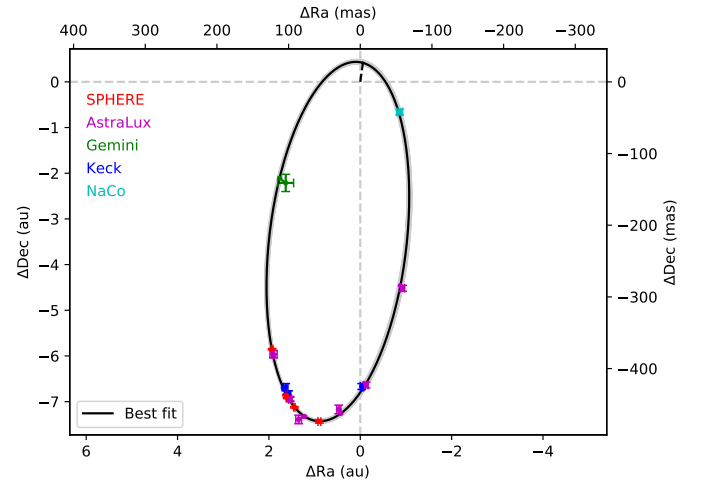
Fig. 5. Plots of a hundred orbits obtained with the MCMC algorithm for system GJ 2060. Astrometric measurements are color-coded according to the instrument, and their position on the fit is also shown. The orbit in black, obtained with the LSLM algorithm, corresponds to the lower \chi^2 .
