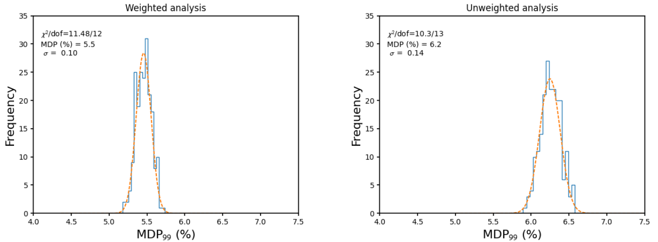
Figure 8. Distribution of \text{MDP}_{99} values for 200 IXPE simulated observations of a point-like source with energy spectrum described by a power-law with number index -2 , a flux 10^{-11} erg/cm 2 /s in the energy range 2–8 keV and 10 days of integration time. \text{MDP}_{99} values are estimated for weighted ( Left ) and unweighted ( Right ) analysis. See text.
