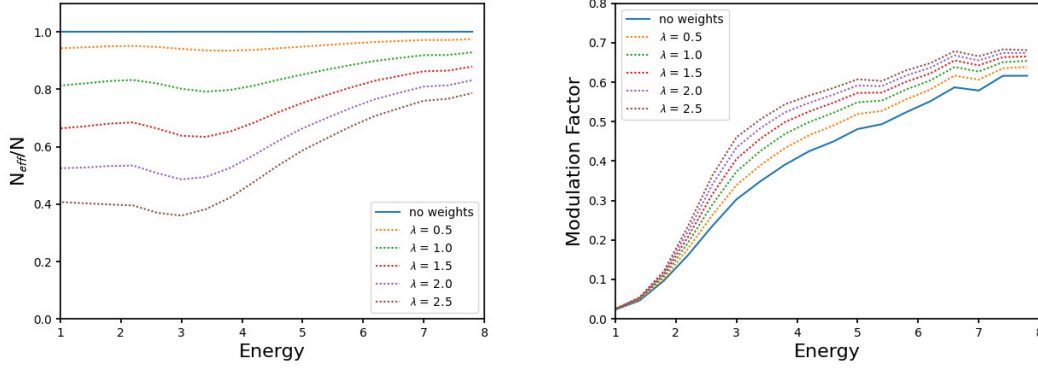
Figure 5. N_{eff}/\mathcal{I} ( left ) and modulation factor ( right ) as a function of the energy at different \lambda values, as obtained by Monte Carlo simulations. See the text.
