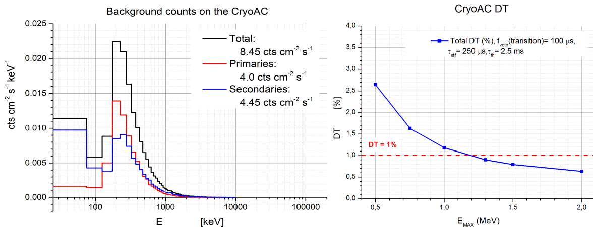
Figure 3. Left – Distribution of the expected energies deposited in the CryoAC absorber (500 \mu m thick Silicon). Right - Expected DT vs the E_{max} for \tau_{th} = 2.5 ms and veto time in transition regime ( t_{veto} ) equal to the pulse peaking time (Color figure online).
