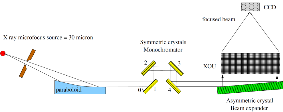
Figure 5. Optical layout of the BEaTriX X-ray test facility.
