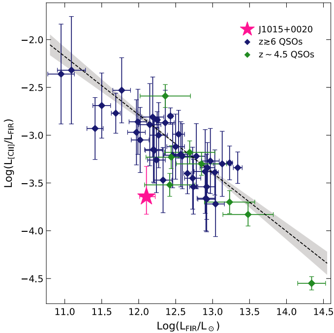
Fig. 5. Ratio of L_{\text{[CII]}}/L_{\text{FIR}} as a function of L_{\text{FIR}} for J1015+0020, compared to high- z QSOs from literature (see Sect. 4 for details) with relative errors. For sources whose uncertainty on L_{\text{FIR}} was not available, we assume the average value of the sample. J1015+0020 is indicated by the magenta star, while blue (green) symbols refer to z \geq 6 ( z \sim 4.5 ) QSOs. The best fit relation obtained from orthogonal linear regression and its 1\sigma error are shown by the dashed line and shaded area.
