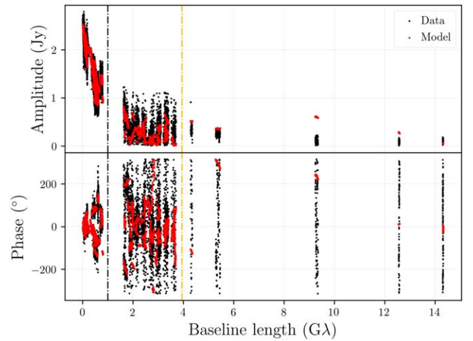
Figure 3. Self-calibrated visibility amplitudes and phases as a function of uv-distance of the RadioAstron observations of OJ 287 on 2014 March–April at 22 GHz. Over-plotted in red is the fit to these data of the CLEAN model obtained from the hybrid mapping using only the data collected during the perigee session, with fringe detections up to a projected baseline length of 3.9 Earth diameters (yellow dotted–dashed line). Detections at larger baseline spacing correspond to the long-baseline snapshots. The black dotted–dashed line separates the ground-only baselines from those obtained to the SRT.
