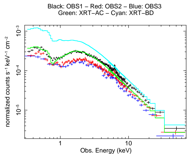
Figure 9. XMM-Newton and NuSTAR spectra (black, OBS1; red, OBS2; blue, OBS3) compared with the two emission states observed during the Swift -XRT monitoring, as analysed in Severgnini et al. (2015, green, low state; cyan, high state).
