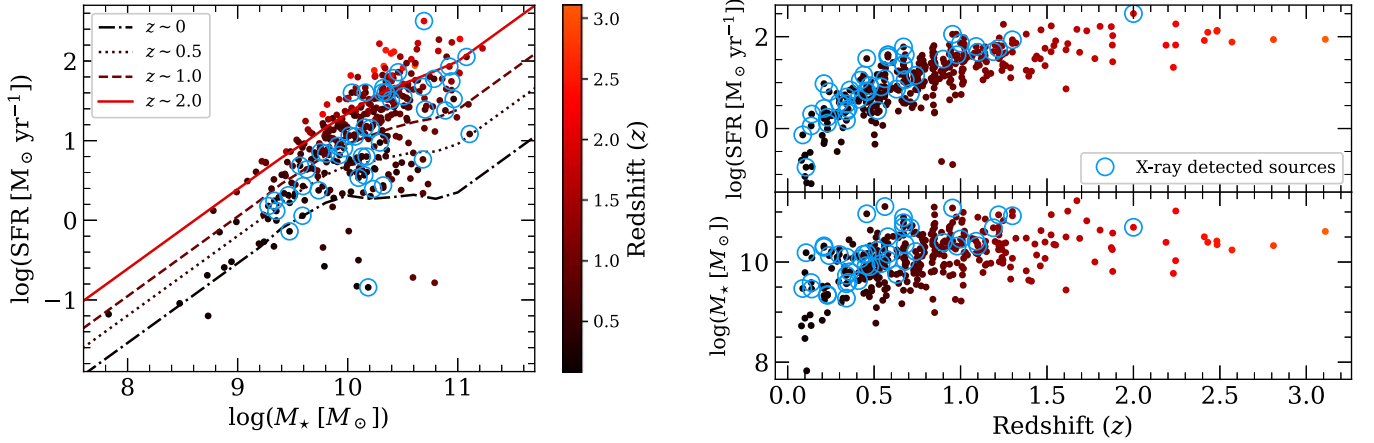
Figure 3. Left: SFR vs. stellar mass ( M_* ) for our final sample of 344 galaxies. The four overlaid curves indicate the locations of the galaxy main sequence for various redshifts that span our sample: z \sim 0 , z \sim 0.5 , z \sim 1.0 , and z \sim 2.0 in the dotted–dashed, dotted, dashed, and solid lines, respectively (Whitaker et al. 2014). The data points and main-sequence curves have been colored by redshift for comparison (see color bar). The blue circled points indicate galaxies that were detected in the X-ray (see Section 3.2). Right: SFR and stellar mass ( M_* ) vs. redshift for our final sample. Similar to the left, the blue circled points are galaxies that were detected in the X-ray (see Section 3.2), which tend to be relatively nearby and of high SFR and M_* .
