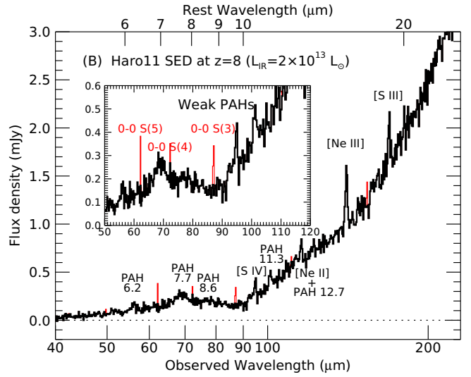
Figure 3. SAFARI 10-hr LR ( R=300 ) spectra for z=8 galaxies simulated for the following three-types of galaxies: (A) HLSJ0918, a HyLIRG at z=5.24 (see Figure 1 and Table 1); (B) Haro 11, a low-metallicity infrared-luminous local BCD that is not infrared-luminous. For HLSJ0918, the L_{\text{IR}} = 10^{11.75} L_{\odot} LIRG SED from Rieke et al. (2009) was used as in Figure 1, while for the two BCDs, the fully-processed Spitzer /IRS low-resolution spectra were obtained from the Combined Atlas of Sources with Spitzer IRS Spectra (CASSIS; Lebouteiller et al. 2011). The infrared luminosities of these SEDs have been scaled to 2 \times 10^{13} L_{\odot} , comparable to the intrinsic luminosity of HFLS3. See the caption of Figure 1 for how these SAFARI spectra were simulated. The red lines show simulated \text{H}_2 emission lines (assumed to be unresolved) produced by 2 \times 10^{10} M_{\odot} of T=200 K gas and 2 \times 10^8 M_{\odot} of T=1000 K gas under the LTE assumption (an ortho-to-para ratio of 3:1 is also assumed). These \text{H}_2 lines are hardly visible in the original galaxy spectra.
