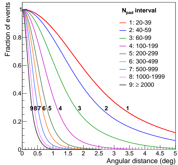
Figure 2. Angular resolution for different N_{pad} intervals, according to simulations. The curves represent the fraction of events beyond the angular distance d from the source, as a function of d .
