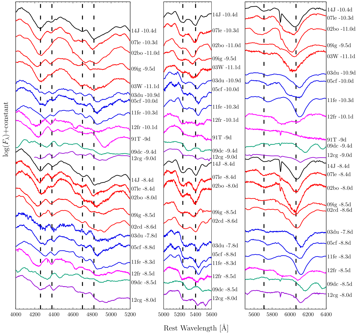
Figure 11. Spectral evolution of SN 14J and some comparison SNe in the wavelength ranges of 4000–5200 Å, 5000–5600 Å, and 5500–6400 Å, at \sim -10 d. Vertical dash lines are overplotted to mark the absorption troughs in SN 14J. The red, blue, magenta spectra represent those of the HV, NV, 91T-like subtypes, respectively. The green and purple lines are for SNe 2009dc (Super-Chandrasekhar Candidate) and 2012cg (99aa-like). Spectra of SNe 1991T (Filippenko et al. 1992), 2002bo (Benetti et al. 2004), 2002cd (B12), 2003W (B12), 2003du (Stanishev et al. 2007), 2005cf (Wang et al. 2009b), 2007le (B12), 2009dc (Taubenberger et al. 2011), 2009ig (Marion et al. 2013), 2011fe (Pereira et al. 2013), 2012cg (Silverman et al. 2012b; Marion et al. 2016), 2012fr (Childress et al. 2013) are used.
