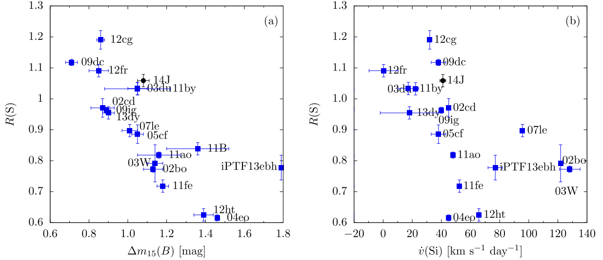
Figure 13. (a) The ratio of S II \lambda 5468 and S II \lambda 5640 absorptions, R(S) versus \Delta m_{15}(B) for some well-observed SNe Ia. (b) The correlation of R(S) versus the velocity gradient \dot{v}(\text{Si}) for the same sample.
