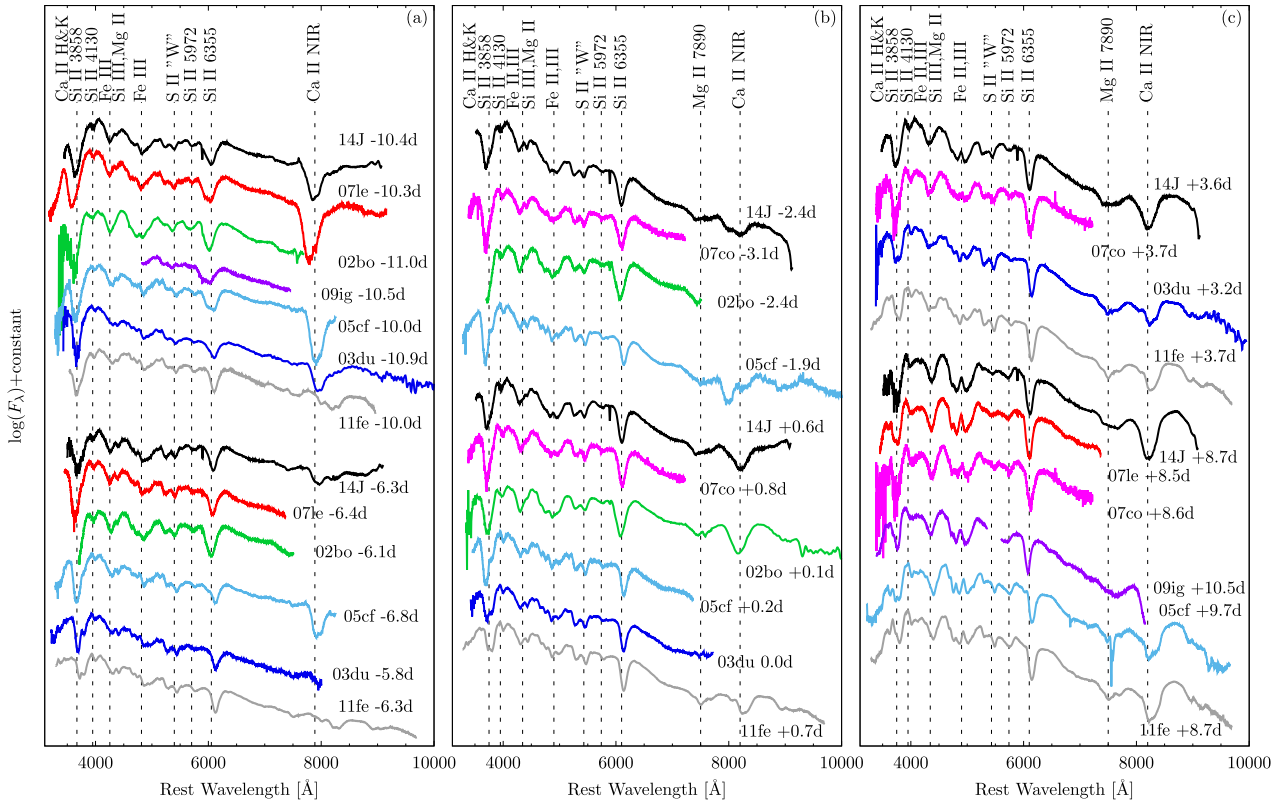
Figure 2. Spectral comparison of SN 2014J with some normal SNe Ia with similar \Delta m_{15}(B) , such as SNe 2002bo, 2003du, 2005cf, 2007co, 2007le, 2009ig, and 2011fe, from \sim -10 to \sim +9 d. All the spectra are de-reddened. An extinction of E(B - V) = 1.23 and R_V = 1.46 for SN 2014J (Marion et al. 2015) is adopted.
