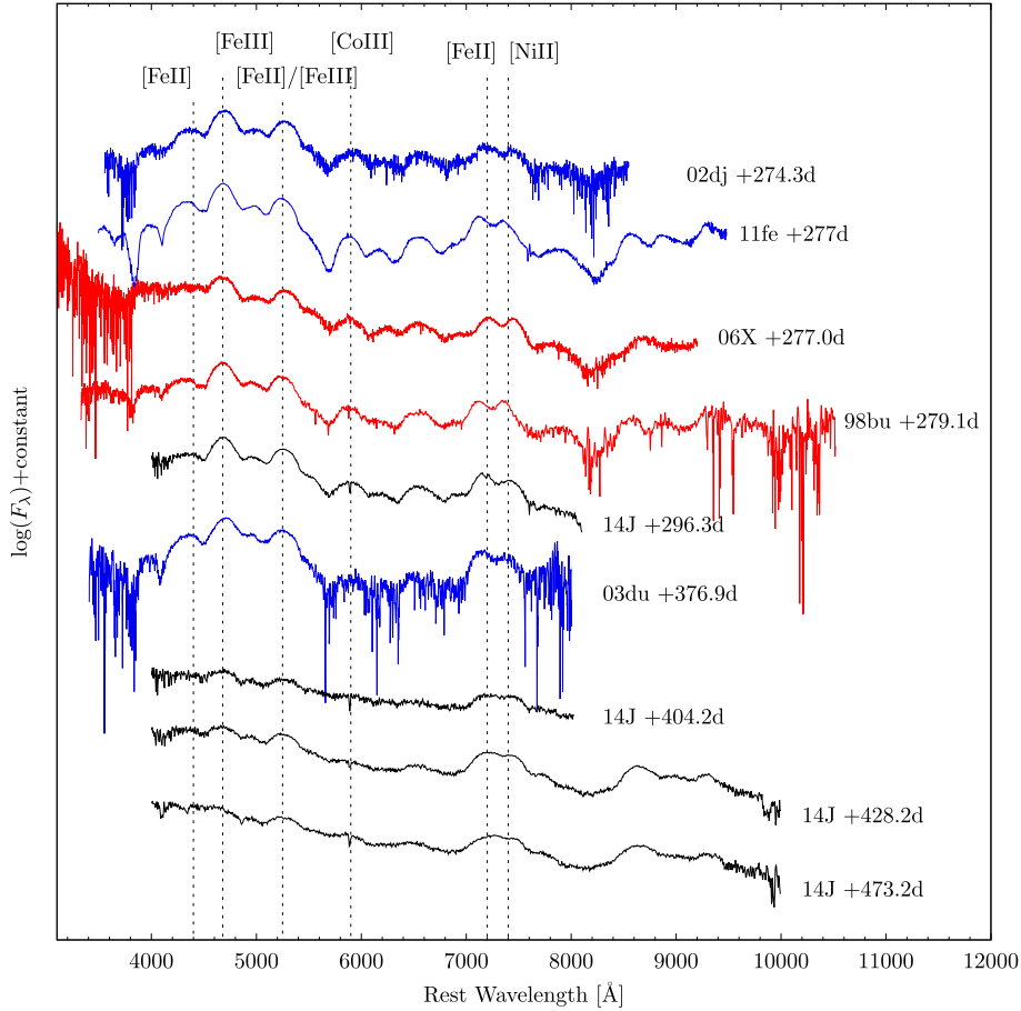
Figure 6. Late-time ( t > +250 d) spectra of SN 2014J (in black), compared with some SNe with (red) and without (blue) light echo detections. The spectrum of SN 2014J at t = +296.7 d is binned by 30 Å. All the spectra are de-reddened. An extinction of E(B - V) = 1.23 and R_V = 1.46 for SN 2014J (Marion et al. 2015) is adopted.
