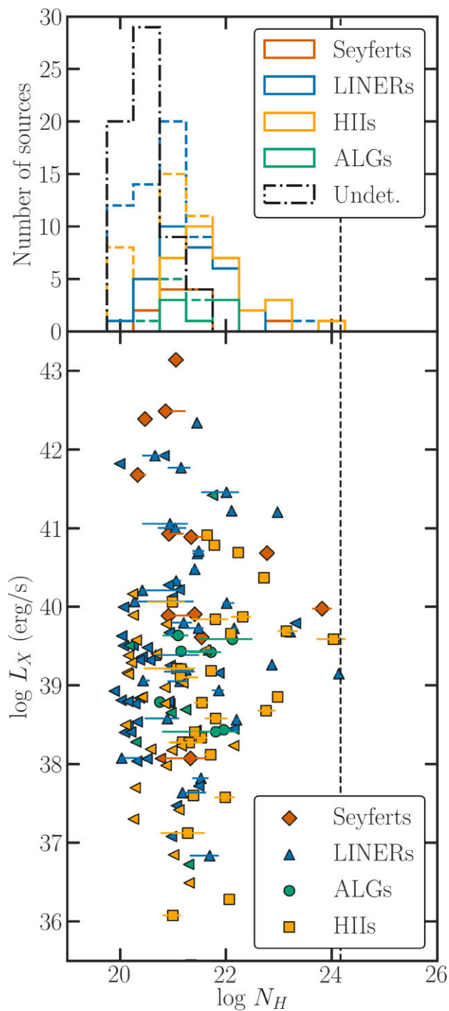
Figure 12. The X-ray luminosity of the entire X-ray sample as a function of absorbing column ( N_H ). For sources with detection significances between 3 and 5 \sigma in the image, we fixed the photon index to 1.8 and obtained a host galactic absorption (see Section 3). For the objects with luminosities >5\times the detection significance in their image, we used the best-fitting values, summing together all neutral absorbers and report in this plot the total absorption from the fits. We also show in the top panel the Galactic absorption along the line of sight to the galaxy for the undetected sources. We show histograms of the N_H distribution for detected sources, where we could constrain the absorbing column by AGN type (solid lines) and all sources including upper limits by AGN type (dashed lines). In the bottom panel, we split the sources by AGN type. In all cases, left pointing triangles denote upper limits. In both panels, we draw a black dashed line which denotes our ‘Compton-thick’ definition, of which no sources are to the right of this line, although some other sources do have values that are close to or their uncertainties pass over this line.
