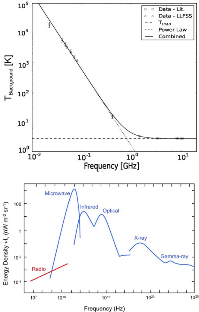
Figure 1. Top: the radio sky zero level in radiometric temperature units, reproduced from Dowell & Taylor (2018), as measured by several different instruments or surveys reporting an absolute zero-level calibration. The spectrum has a power law at frequencies below \sim 10 GHz above the CMB level. Results are shown for ARCADE 2 at 3–10 GHz (Fixsen et al. 2011), Reich & Reich (1986) at 1.4 GHz, Haslam et al. (1982) at 408 MHz, Maeda et al. (1999) at 45 MHz, and Roger et al. (1999) at 22 MHz, as well as several points reported by Dowell & Taylor (2018). Bottom: the photon backgrounds in the universe in units of spectral energy surface brightness density. Reproduced from Singal et al. (2018).
