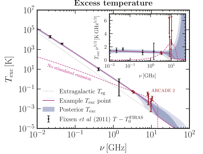
Figure 16. Point-wise posterior for T_{\text{exc}} within our proposed model, showing the middle 68% and 95% regions (dark and light blue regions, respectively). We include the contribution from unresolved extragalactic sources T_{\text{eg}} (dashed gray—Gervasi et al. 2008) for completeness. The spectrum for a single point in parameter space is shown in pink. Radio data, plotted as T - T_0^{\text{FIRAS}} , include measurements from ARCADE 2, shown in red (Fixsen et al. 2011), with results from other telescopes shown in black. The pink dashed line shows a fit to the ARCADE 2 data only assuming no stimulated emission.
