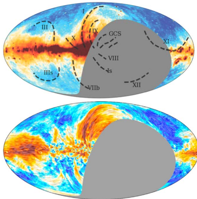
Figure 5. C-BASS North maps of total intensity (top) and polarized intensity (bottom) in Galactic coordinates using a Mollweide projection. The total intensity map color scale has been saturated along the Galactic plane and includes the locations of well-known radio loops (Vidal et al. 2015). The polarized intensity map has the projected B-field direction overlaid using line-integral convolution.
