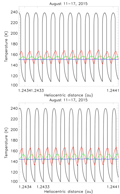
Figure 9. Case 1 (upper panel) and Case 2 (lower panel), location B, 2015 August 11–17: temperatures on the surface (black line) and in the layers below the surface (red line, 2.5 cm; green line, 5 cm; blue line, 10 cm).
