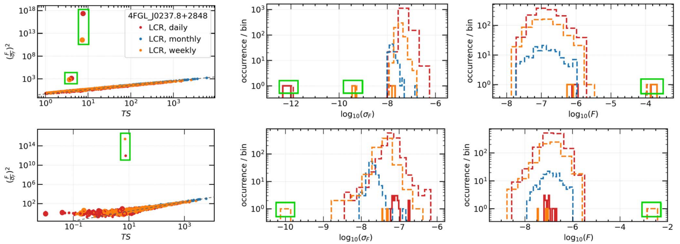
Figure 8. Example of validation plots for the FSRQ 4C +28.07. The top panels show the case for which the spectral index ( \alpha for this source) is fixed. In all plots we are considering the 0.1–100 GeV energy range. The bottom panels show the case for which the spectral index is free to vary. The ratio of the flux to the flux uncertainty (left panels) is expected to be approximately proportional to the square root of TS. The middle panels show the distributions of the flux statistical uncertainties. Flux distributions are shown in the right panels. In this example, the distributions are good except for the outliers highlighted within green squares, which should be either further investigated or removed. In the histograms, the dashed lines represent the results from all time bins. The solid lines represent bins that did not converge. Notice that outliers are not necessarily the results from analyses that did not converge.
