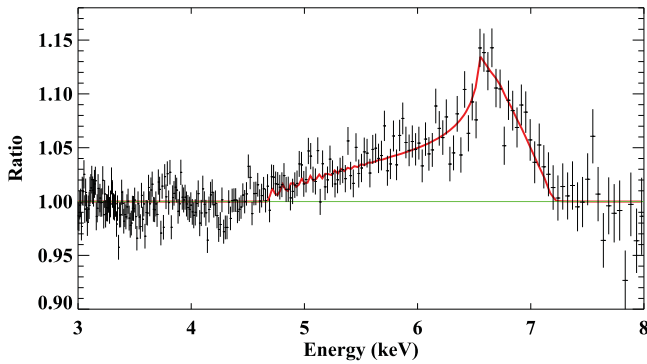
Figure 3. Fe line profile of Serpens X-1. The spectrum is modeled as tbabs (bbody + power-law + diskline) , and the plot is produced by setting the normalization of DISKLINE to be 0. The plot is visually binned with “ seplot rebin ” in XSPEC . The bin sizes through the Fe line are \sim 0.042 keV. The red line shows model. It can be seen that the DISKLINE model fits the asymmetric line very well.
