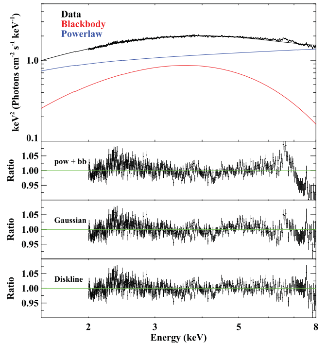
Figure 2. Top panel: the unfolded spectrum of Serpens X-1 with decomposed model components. We display the data/model ratios of the continuum model \text{tbabs}*(\text{bbody} + \text{power-law}) Model 3, and Model 3a in the lower panels.
