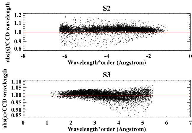
Figure 7. Order-sorting region of chips S2 and S3. The x-axis is the wavelength times order, and the y-axis is the absolute value of x-value over the CCD wavelength. The figure shows the selected events during the order-sorting process. The mild curvature shown in S3 might be the cause of discrepancy between the HEG \pm 1 spectra.
