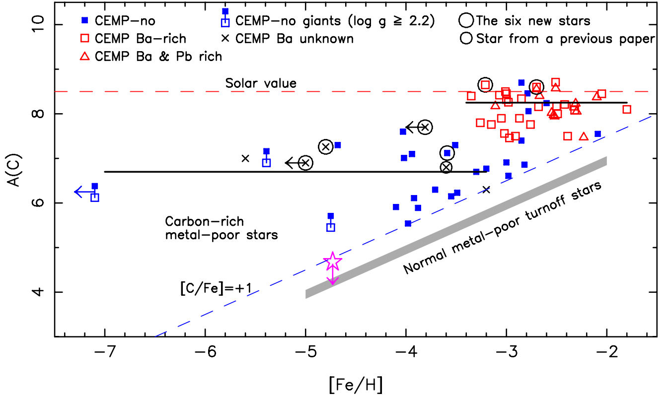
Fig. 6. Carbon abundances A(\text{C}) of CEMP stars as a function of [\text{Fe}/\text{H}] . The stars in the present paper and in Caffau et al. (2013a) are shown with big and small circles, respectively. The other turn-off stars come from the literature (Sivarani et al. 2006; Frebel et al. 2005, 2006; Thompson et al. 2008; Aoki et al. 2008; Behara et al. 2010; Masseron et al. 2010, 2012; Yong et al. 2013; Cohen et al. 2013; Li et al. 2015). The CEMP-no turn-off stars are represented by filled blue squares. The CEMP-no giants are represented by two symbols: an open blue square for the measured value of the C abundance, and a filled blue square for the empirically corrected (for the first dredge-up) A(\text{C}) value. The CEMP-s or -rs stars are indistinctly represented by open red squares, but by open red triangles if they are also Pb-rich. When the Ba abundance is unknown the star is marked with a black cross. The upper limit marked as a violet star is the only “C-normal” star that appears in this plot: SDSS J1029+1729 (Caffau et al. 2012). The solid horizontal (black) lines represent the mean value of the carbon abundance for CEMP stars with [\text{Fe}/\text{H}] > -3.0 ( A(\text{C}) = 8.25 ) and for CEMP stars with [\text{Fe}/\text{H}] < -3.4 ( A(\text{C}) = 6.8 ) as derived by Spite et al. (2013). On the upper A(\text{C}) -band all the stars but four (HE 0007-1832, HE 022-4831, SDSS J0036-1043, and CS 22958-42) are Ba-rich. On the contrary, on the lower A(\text{C}) -band all the stars are CEMP-no.
