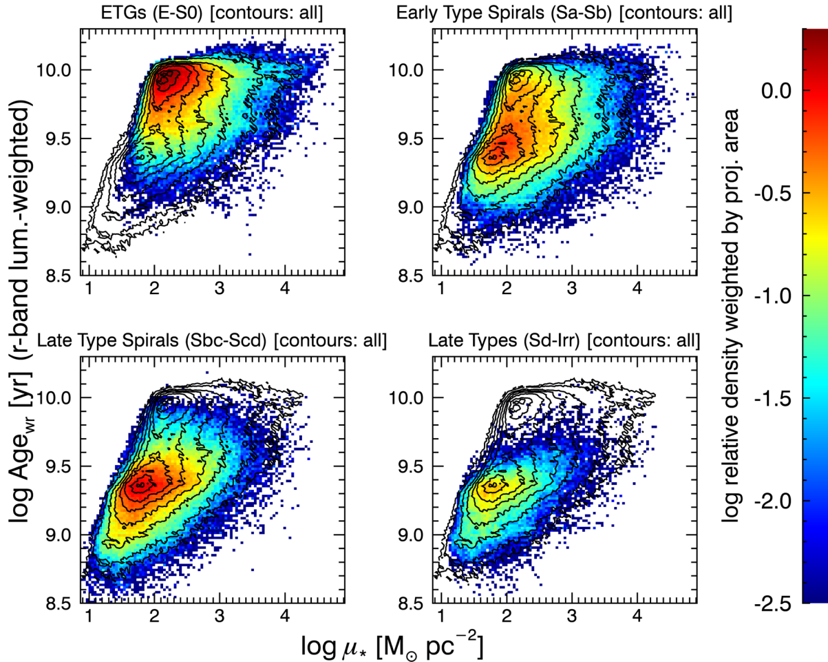
Figure 7. Distribution of regions belonging to galaxies of different morphological classes, volume corrected and weighted by physical projected area, in the \log \mu_* – \log \text{Age}_{\text{wr}} plane. Distributions are normalized as in the overall distribution of Fig. 6, so that the sum of the four panels results in the overall distribution. Contours mark densities that are 0.9, 0.75, 0.5, 0.35, 0.20, 0.1, 0.03 and 0.01 times the maximum density of the overall distribution of Fig. 6.
