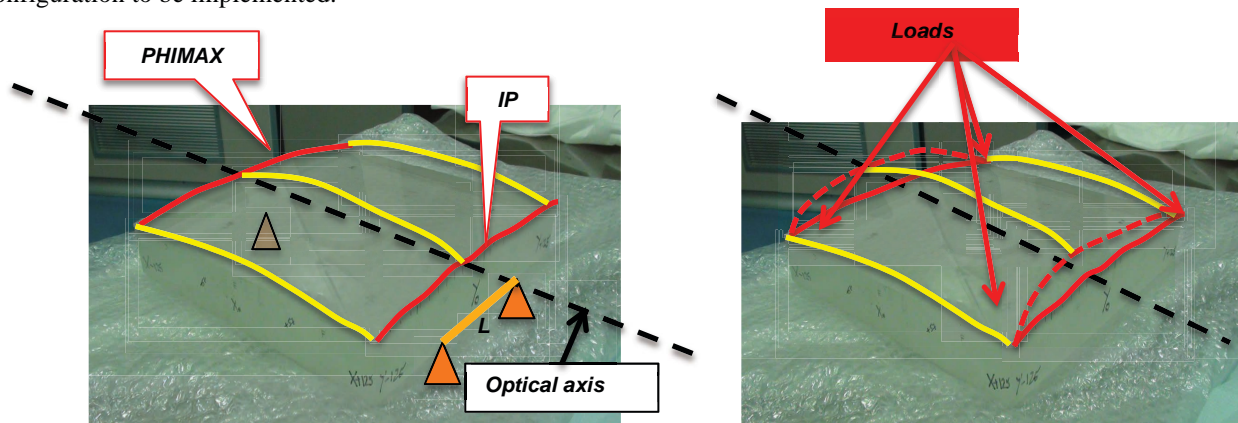
Figure 12: (A) Mold geometry: the radius at PHIMAX and at the Intersection plane (IP) are highlighted in red. The longitudinal profiles on the central and on the lateral side are marked in yellow. (B) The variations in the radius of curvature in and in longitudinal profiles are reported as dashed lines. Red arrows indicate the positions for the loads.
