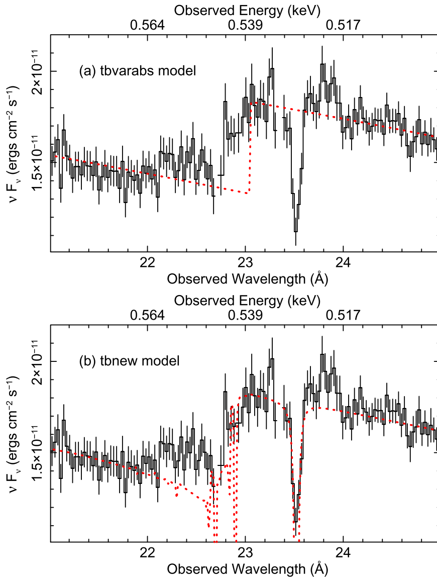
Figure 3. Zoom-in of the fluxed RGS spectrum of Ark 120 in the neutral O–K edge region, due to absorption in the Galactic ISM toward Ark 120. Wavelength (energy) is plotted in the observed ( z = 0 ) frame. The top panel (a) shows the data compared against the TBVARABS absorption model (red dotted line), where a simple O I edge which is not able to correctly account for the absorption in this region. The lower panel (b) shows the comparison against the TBNEW model, which reproduces well the O I K\alpha absorption line at 23.5 Å (or 527 eV), while the drop around the edge below 23 Å is more gradual due to the higher order resonances present in the model. The excess blueward of the O edge is likely due to O VII emission associated with the AGN. Note that the models are superimposed on the spectra that have been fluxed against a \Gamma = 2 power law, but the data are not unfolded against either absorption model.
