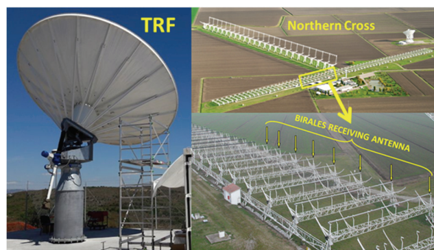
Fig. 1. The BIRALES system composed of the TRF (on the left) and the Northern Cross telescope (on the right).
