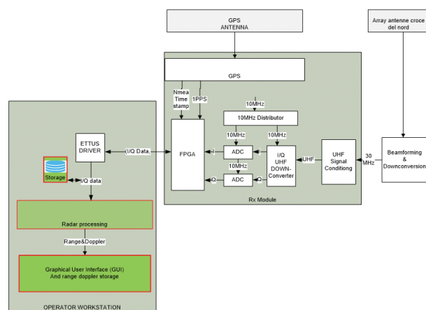
Fig. 4. Receiver architecture
