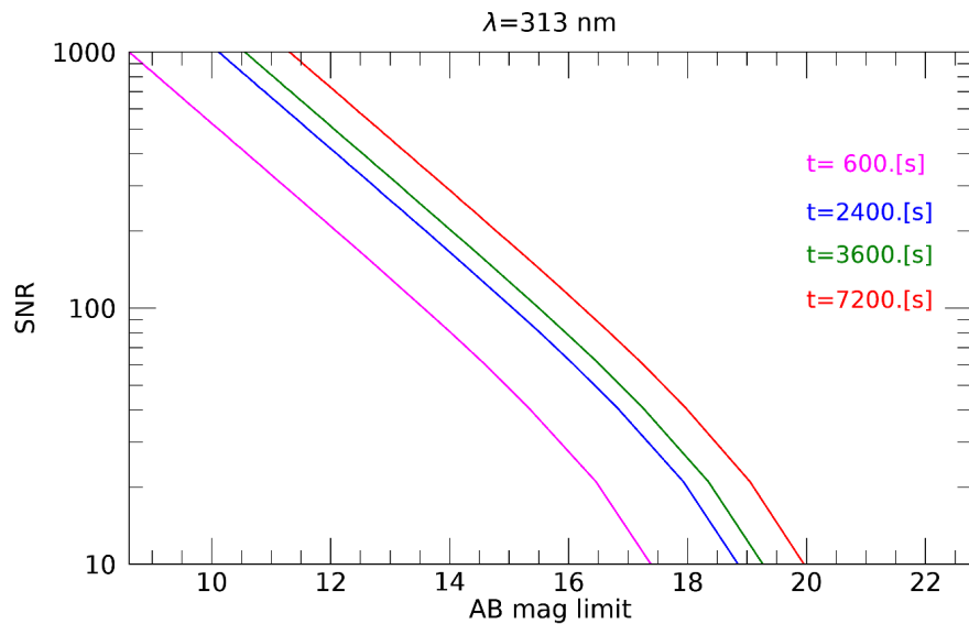
Figure 9. SNR versus magnitude limit (AB unit) at 313nm for different exposure times, in HR-mode, template spectrum with constant AB magnitude, U_{sky} = 22 \text{ mag arcsec}^{-2} , airmass = 1.16, seeing = 0.87'' , dark current = 0.5e^- \text{ pix}^{-1} \text{ hr}^{-1} , RON = 2.5 e^- \text{ rms} , and binning 1x1 pixel.
