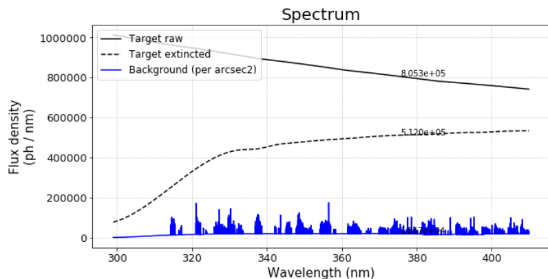
Figure 10. Example of the input spectra in the Basic Version E2E notebook (for a flat spectrum of U = 18 \text{ mag} ). The integrated flux from the target and the sky is computed assuming the collecting area of the primary mirror of a VLT unit telescope and a detector integration time of 3600s. Left : photon balance between the target and the sky background. Right : spectra of target (with extinction) and background.
