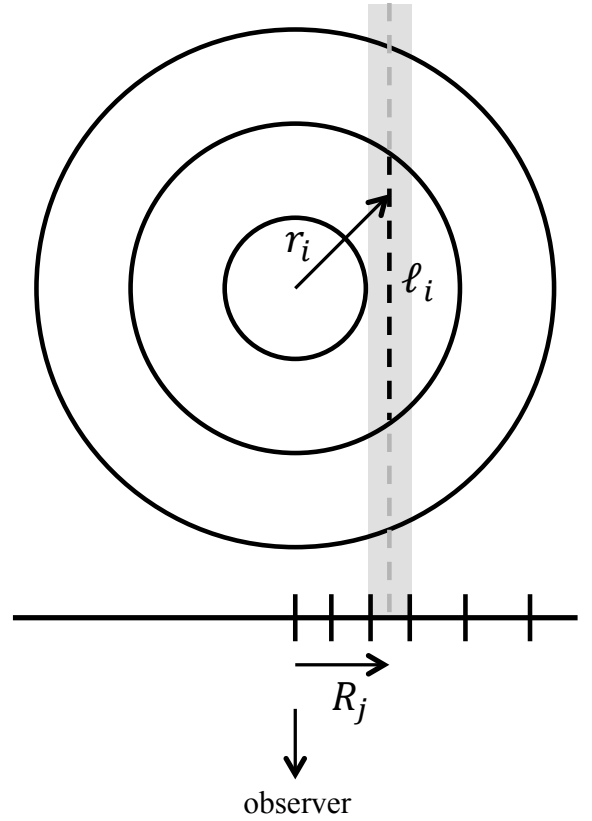
Figure 3. The concentric shell model, adapted from McLaughlin (1999). The observer sees a 2-D map with radial bins denoted by R_j , while the 3-D shells have radii r_i . The radial coordinates for the 2-D bins do not necessarily match those for the 3-D shells. l_i is the distance along the line of sight that radial shell i contributes to the 1D bin at radius R_j .
