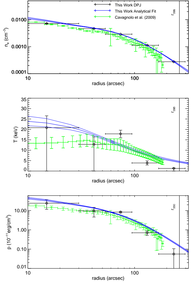
Figure A35. MACS J0717.5+3745. Our profiles for this cluster are in excellent agreement with the profiles obtained in the ACCEPT analysis, and our smooth parametric fit indicates a temperature drop at large radius at a significance of 24\sigma . This cluster has been studied extensively in different wavelengths. Ma et al. (2009) found that the cluster consists of four large subclusters based on X-ray imaging and galaxy positions. Through lensing ( Medezinski et al. 2013 ; Diego et al. 2015 ; Limousin et al. 2016 ; Umetsu et al. 2016 ), four large masses are also clearly found, reflecting that this cluster is a complex merger. Mroczkowski et al. (2012) studied this cluster through the SZ effect, X-ray and lensing observations. They also found very hot gas near 30 keV in some regions of the cluster. A large kSZ signal in one of the subclusters, which has not been accounted for in our analysis, could potentially be a source of bias in our results ( Sayers et al. 2013c ).
