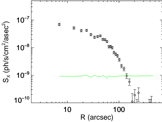
Figure 2. Example X-ray surface brightness profile (MACS J0416.1-2403). The green line represents the background level, and the black points are the the estimated surface brightness after subtracting the background.
