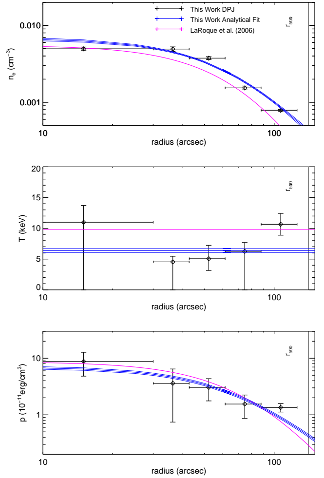
Figure A43. MS1054.4-0321. Compared to the smooth parametric fits of LaRoque et al. (2006), our smooth parametric fits show a significant offset in both density and temperature. Gioia et al. (2004) used XMM-Newton to find an average temperature of \sim 7\text{keV} , in good agreement with our results. Neumann & Arnaud (2000) studied this cluster using the X-ray ( ROSAT ), finding substructure and other signs of recent merging processes (e.g., BCG and X-ray peak offset, X-ray centroid and peak offset).
