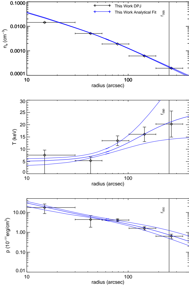
Figure A16. MACS J1115.8+0129. The ACCEPT analysis finds densities systematically lower than ours, but our results are consistent with other studies (e.g., Mantz et al. 2016), and so the ACCEPT profiles are not plotted. Donahue et al. (2014) found temperature profiles from X-ray spectroscopy ( XMM-Newton and Chandra ), showing a central temperature of around 3 keV rising to 8–9 keV, roughly matching our results over the same region. However, the XMM-Newton data then show a decrease in the temperature profile near 800 kpc (160''), which is not seen in our results.
