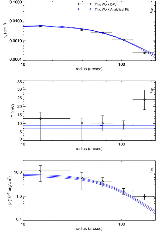
Figure A23. MACS J0416.1-2403. Several studies have identified this cluster as a binary merger system. Mann & Ebeling (2012), using optical and X-ray data, found this system to contain a possible binary head-on collision, just after the first collision. Jauzac et al. (2015) conducted a joint X-ray and optical study, and unveiled a large structure associated with a line-of-sight filament that could not be seen in the X-ray. A large offset in the radial velocity between two subclusters was found, and their temperatures were determined to be 10 and 13.6 keV, slightly higher than our isothermal smooth parametric fit. Ogrea et al. (2015) created temperature, pressure, and entropy maps using a multi-wavelength analysis of Chandra , the VLA, the GMRT, and Hubble . The temperature map is elongated, and has a relatively high mean temperature of 10 keV. The radio halo is also elongated along the same direction.
