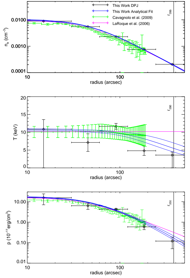
Figure A11. Abell 697. We find a relatively flat inner temperature profile, and we detect a drop in temperature near r_{500} at a significance of 4.5\sigma . Our Pressure profiles are consistent with the joint X-ray/SZ study of LaRoque et al. (2006), and there is good agreement between our density, temperature, and pressure profiles and the corresponding ACCEPT profiles. Although we characterized the cluster as non-disturbed, several other studies have shown that the cluster has undergone recent merging. Girardi et al. (2006) conducted a multi wavelength study using optical and X-ray data, where line of sight galaxy velocity dispersions and spectroscopic temperatures were calculated, respectively, and found that A697 is not relaxed. With elongated X-ray emission and substructures near the center, Abell 697 likely went through many mergers. Through lensing, Metzger & Ma (2000) also concluded that the cluster has undergone a recent merger.
