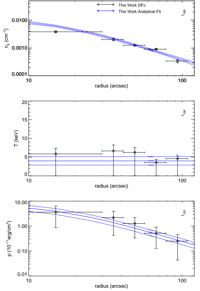
Figure A39. MS 2053.7-0449. This is the least massive cluster in our sample, with M_{500} \approx 3 \times 10^{14} M_{\odot} , and one of the dimmest clusters in the SZ. The low mass and high redshift also produce a weak X-ray signal. This makes it one of the few clusters in our analysis where the constraints do not extend to r_{500} . Verdugo et al. (2007) found a bimodal and elongated mass distribution for this cluster using Hubble data, indicating a merger.
