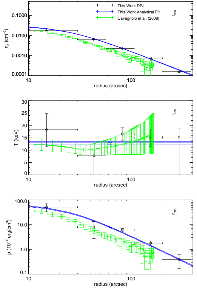
Figure A21. MACS J2211.7-0349. Our densities and pressures are systematically and significantly higher than those found in the ACCEPT study. Due to the lack of independent results for this cluster, it is not possible to determine which analysis may be in error.
