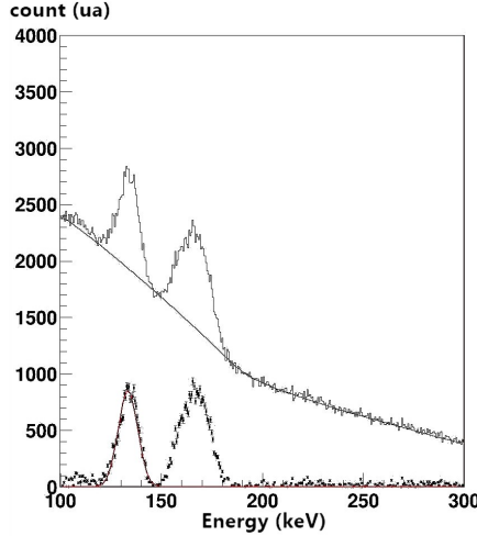
Figure 17. Measured delayed spectrum with a H 2 +O 2 (0,3%) gas mixture in the target. Muonic Oxygen X-rays: 133 keV K_{\alpha} , 158 keV K_{\beta} and 167 keV K_{\gamma} lines, with background (top) and background subtracted (bottom). The energy resolution for the 133 keV line is 8.5%.
