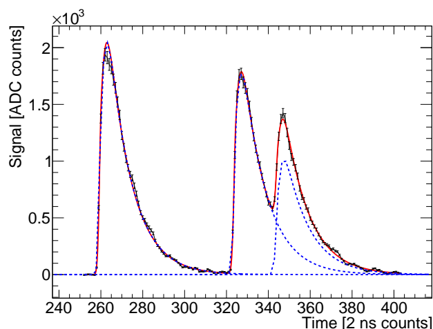
Figure 12. Example of multiple overlapping signals. Black points represent the data waveform, red line is a fit of the data using three signal shapes shown as blue lines.
