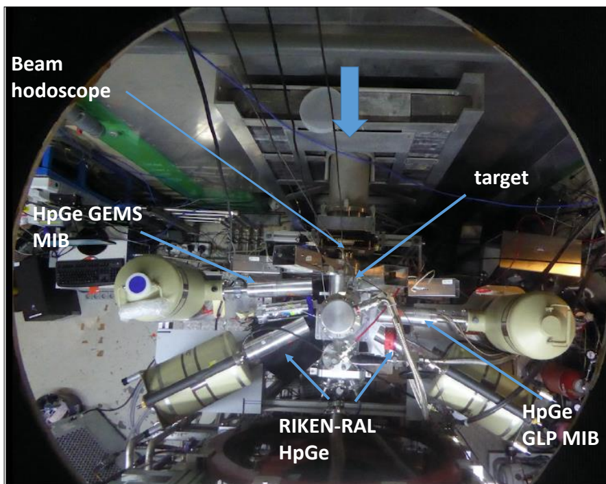
Figure 10. Picture of the FAMU layout seen from the top. The position of the HPGe detectors and the 1 mm pitch beam hodoscope are shown.
