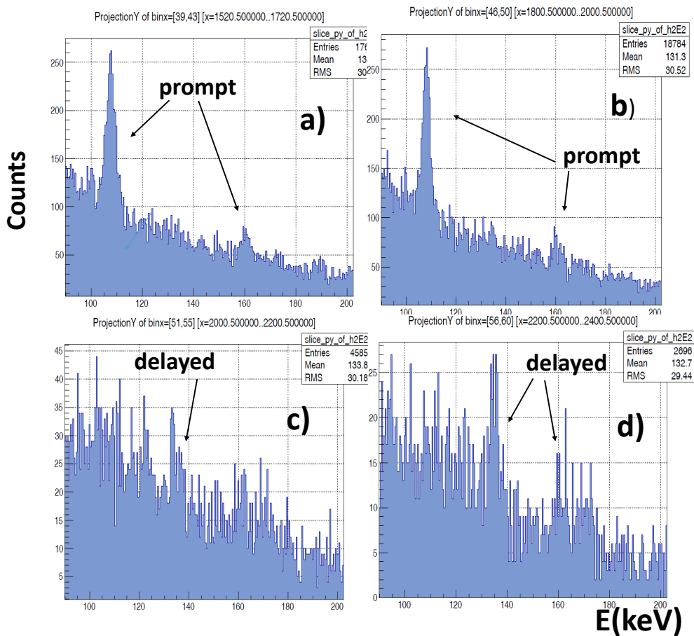
Figure 23. Time evolution of the K_\alpha(2p \rightarrow 1s) line energy distribution, as reconstructed from the GEM-S HPGe detector, in four time slices. (a) 1520–1720 ns, (b) 1800–2000 ns, (c) 2000–2200 ns and (d) 2200–2400 ns.
