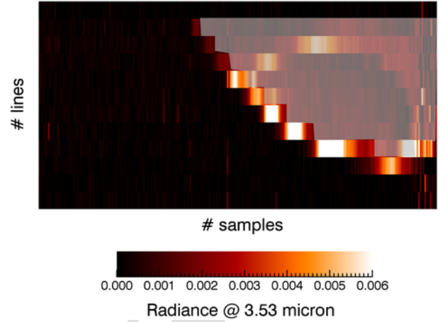
Fig. 1. Example of JIRAM image (n. 160,826–175,419) acquired by the spectrometer. The radiance at 3.53 \mu\text{m} is plotted as a function of the samples (pixel) number and lines number. Each line represents one slit acquisition. The shaded area indicates the limit of the Jupiter disk at 1-bar; all pixels outside this region correspond to the \text{H}_3^+ emission originated from regions above the Jupiter disk.
