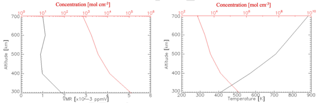
Fig. 6. Correlation of VMR and H_3^+ concentration (image on the left) and between temperature and H_3^+ concentration (image on the right), retrieved with our inversion code. The scale for VMR and temperature are shown in the lower x-axis, while in the upper one there are the values for concentration in log-scale (in red). Data at all available latitudes were averaged. (For interpretation of the references to colour in this figure legend, the reader is referred to the web version of this article.)
