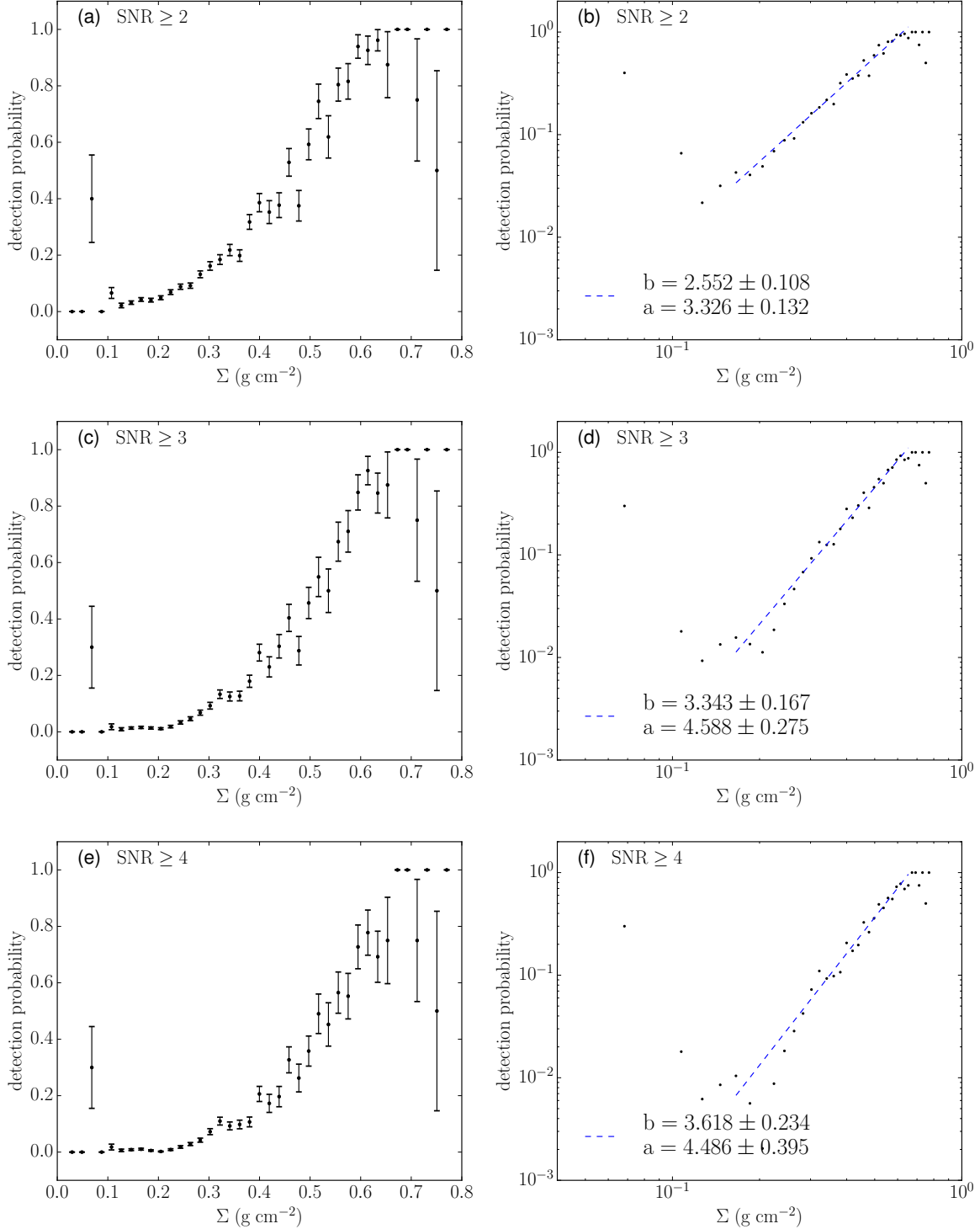
Figure 3. (a): 1.3 mm continuum detection probability P_{1.3\text{mm}} as a function of \Sigma . Here the continuum detection threshold is SNR = 2 with the RMS noise being 0.2 mJy per 2'' beam. The error bars are the square root of the variance of the Bernoulli distribution (see text). (b): The same as panel (a), but in logarithmic scale. The blue dashed line shows a power-law fit over the indicated range of \Sigma . The parameters a and b follow equation 3. (c): Same as (a), but with a detection threshold of SNR = 3. (d): Same as (c), but in logarithmic scale. (e): Same as (a), but with a detection threshold of SNR = 4. (f): Same as (e), but in logarithmic scale.
