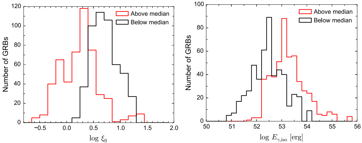
Figure 5. Distribution of \xi_0 (left) and E_{\gamma,\text{iso}} (right) for a trial simulation ( t_{p,\text{opt}} = 1000 s, peak mag = 18 mag, observed frequency = 10 GHz, k = 0 ) for fluxes above and below the median. Bursts with above-median fluxes in the radio have larger energies and smaller \xi_0 (closer to thick-shell regime), helping to mitigate the effects of the numerical corrections.
