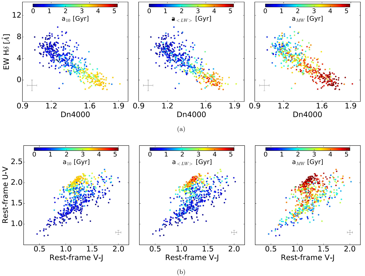
Figure 5. EW(H\delta) vs. D_n4000 (upper panel) and U - V color vs. V - J color (lower panel) color-coded by the time after which the final 10% of stars were formed (left), the mean light-weighted age (middle), and the mean mass-weighted age (right). Typical error bars are indicated in gray.
