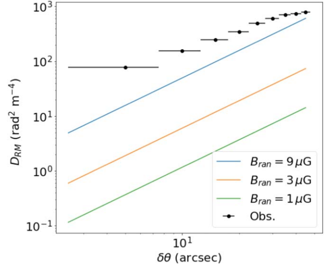
Figure 6. Structure functions of the RM for G21.5–0.9. The black dots are the observational results calculated from the RM map in Figure 4. The colored lines show the theoretical model with different strengths of magnetic fluctuation (Minter & Spangler 1996).
