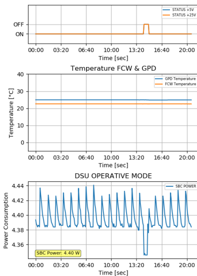
Fig. 7-19: Power off of the 25 V after the detection of an over threshold on the Vdrift HV.
