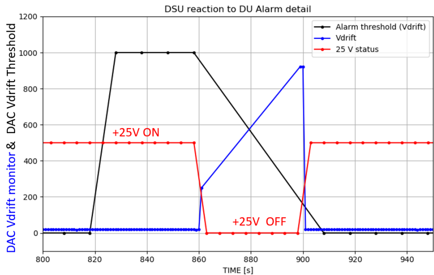
Fig. 7-19: Power off of the 25 V after the detection of an over threshold on the Vdrift HV.
