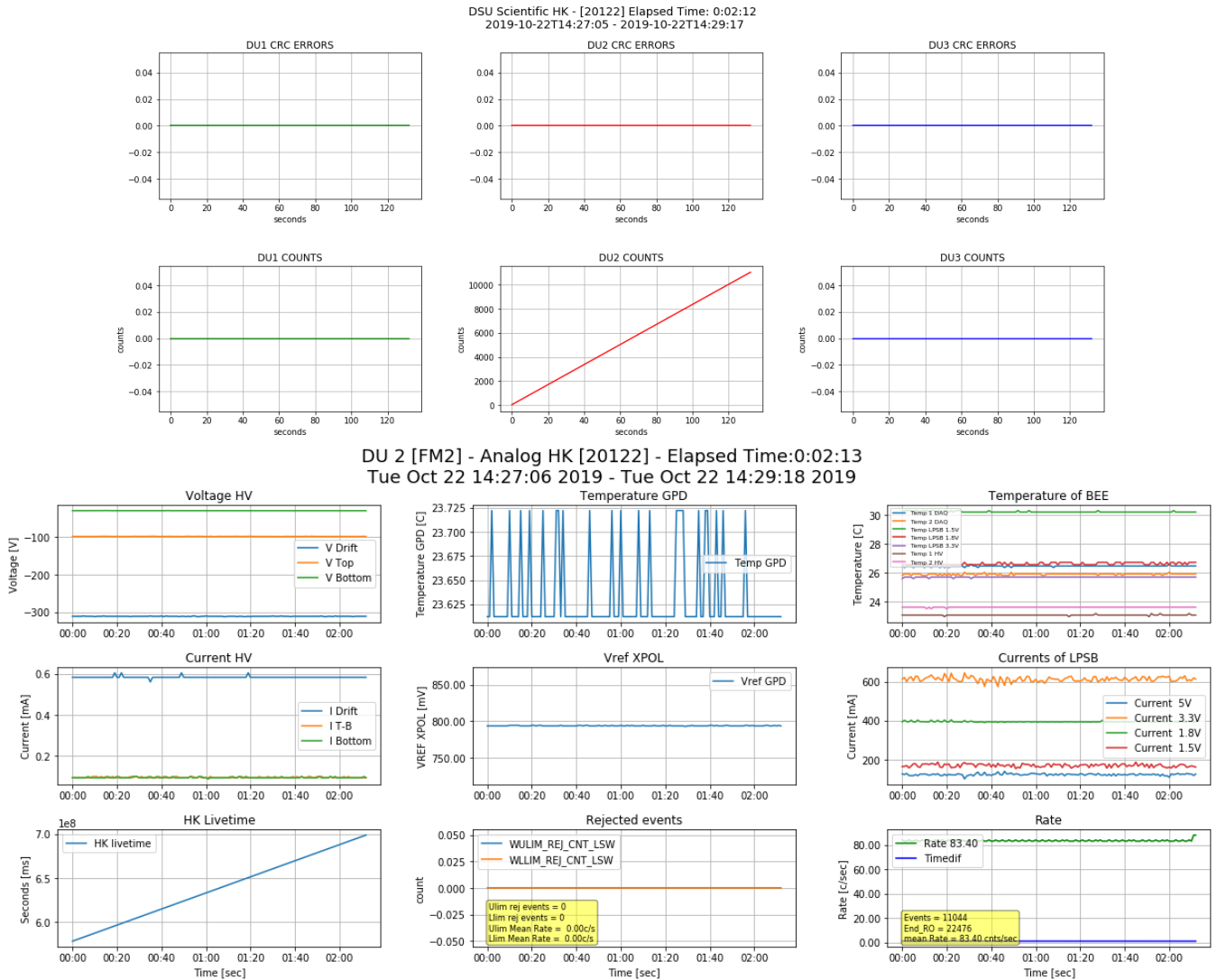
Fig 7-8: DSU Scientific Ratemeters (APID 1203) and DU FM2 HKs (APID 1322) during the DU Charge Injection Procedure (sec. 7.7).
