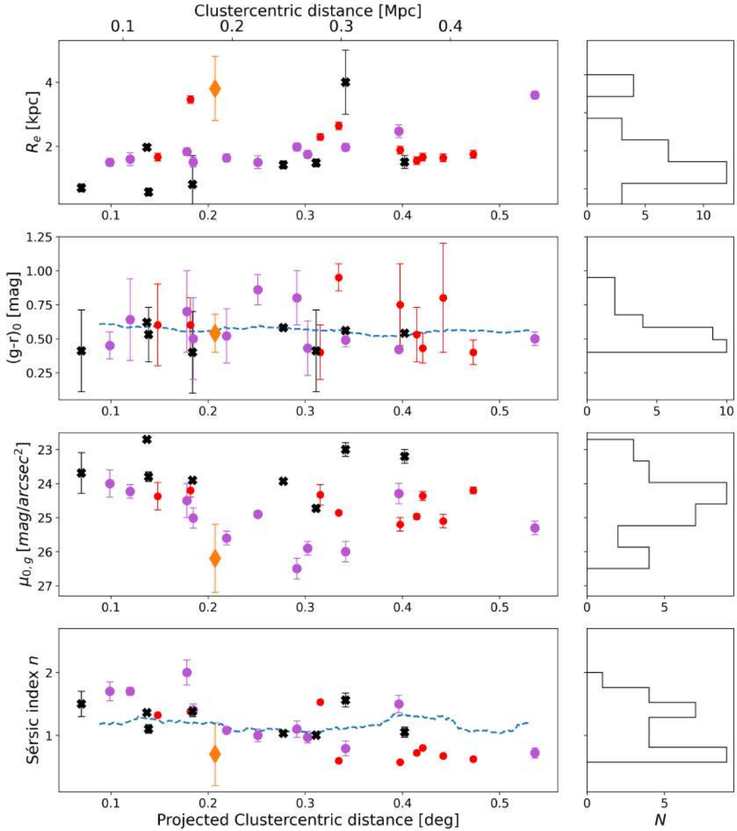
Fig. 7. Left panel: structural parameters for UDGs (purple circles are UDGs in this work, red circles are UDGs from Iodice et al. 2020, and the orange diamond marks UDG 32 Iodice et al. 2021) and LSB galaxies (black crosses) in the Hydra I cluster as a function of the cluster-centric projected distance. From the top to the bottom: effective radius R_e , g-r color, central surface brightness \mu_0 in the g band, and the Sérsic index n . The blue dashed line is the mean locus derived for the dwarf galaxy sample in Hydra I published in Paper I. The running mean shown is calculated considering a moving window of a fixed number of objects (50). Right panel: distributions of the parameters shown in the left panels.
