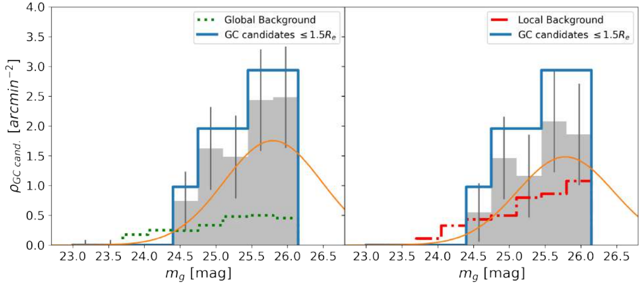
Fig. 5. Total luminosity function of the GC candidates over the joint sample of UDGs and LSB galaxies (Table 3) with N_{GC} \geq 0 within 1.5R_c normalized to the total galaxy area (solid blue line). Left: GCLF globally corrected. The density distribution for the global background is shown with green dotted line. The gray shaded histogram shows the residuals of the two. The solid line shows the best-fit Gaussian function of the GC luminosity function (gray bins). The best-fit parameters are: \mu_{g,TOM} = 25.8 \pm 0.3 mag, \sigma_{GCLF} = 0.69 \pm 0.12 mag. Right: As left panel, but using the local background (red dot-dashed line). The best-fit parameters are: \mu_{g,TOM} = 25.8 \pm 0.2 mag, \sigma_{GCLF} = 0.66 \pm 0.14 mag. The error bars show the uncertainties on the residual GC density calculated as detailed in Sect. 4.
