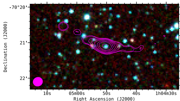
Figure 21. ASKAP ESP image of the FR-I AGN. The background image is a three-colour IRAC composite with 8.0, 4.5, and 3.6 \mu\text{m} represented as red, green, and blue, respectively. The magenta radio contours are from our 1320 MHz survey drawn at 0.25, 0.3, 0.5, 0.7, 1, 1.5, 2, 3, and 5 \text{mJy beam}^{-1} . The 1320 MHz beam size of 16.3 \times 15.1 \text{ arcsec}^2 is shown as a filled magenta ellipse in the lower left corner.
