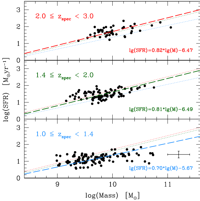
Fig. 19. SFR vs. Mass in three redshift bins, each spanning \sim 1.2 Gyr. For each galaxy, the plotted SFR estimate is \text{SFR}_{\text{IR+UV}} for IR-detected galaxies and \text{SFR}_{[\text{OII}]} or \text{SFR}_{\text{UV}} for galaxies with no IR data respectively in the [OII] sample and in the UV sample. In each panel the three lines are the fits (OLS bisector) to the data in the three redshift bins. Different colours identify each redshift bin.
