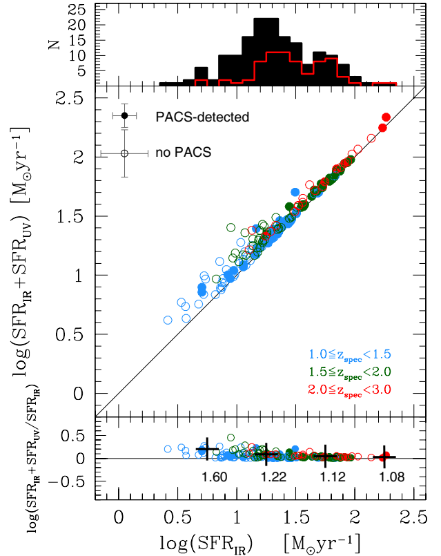
Fig. 10. Main plot: comparison between SFR_{\text{IR+UV}} and SFR_{\text{IR}} for SFGs with at least one IR detection. Filled points mark PACS-detected galaxies. Bottom plot: SFR_{\text{IR+UV}} over SFR_{\text{IR}} ratio as a function of SFR_{\text{IR}} . Median ratio in bins of SFR_{\text{IR}} are also shown. Upper plot: black histogram is the distribution of SFR_{\text{IR}} over the entire sample of SFGs; red empty histogram is the distribution of PACS-detected sources only.
