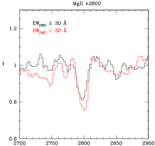
Fig. 16. Composite spectra of galaxies in the [OII] sample in two bins of rest-frame EW_{[\text{OII}]} : zoomed-in image of the \text{MgII}\lambda 2800 ISM absorption line.
