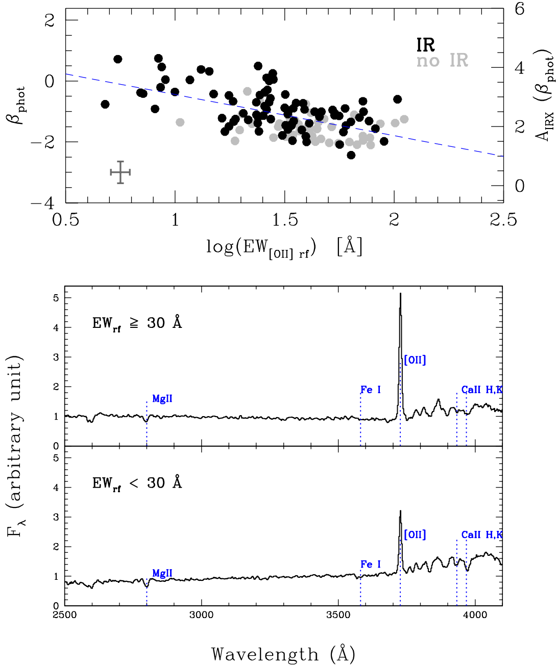
Fig. 15. Top: \beta_{\text{phot}} vs. \log(EW_{[\text{OII}]}) rest-frame. We use the convention of positive EW for emission lines. The right axis converts \beta_{\text{phot}} to A_{\text{IRX}} using Eq. (11). Black points represent IR-detected galaxies, while grey points represent galaxies with no IR detection. The blue dashed line is a linear fit to the points. Bottom: average spectra in two bins of rest-frame EW_{[\text{OII}]} . Lines of interest are labelled.
