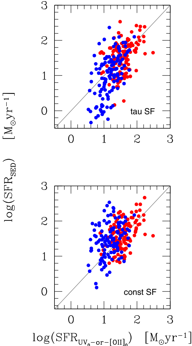
Fig. 18. Comparison between \text{SFR}_{\text{SED}} and SFR estimated from spectroscopic tracers: UV flux, corrected using \beta , for galaxies in the UV sample (red points), and [OII] \lambda 3727 flux, corrected using \text{EW}_{[\text{OII}]} , for galaxies in the [OII] sample (blue points).
