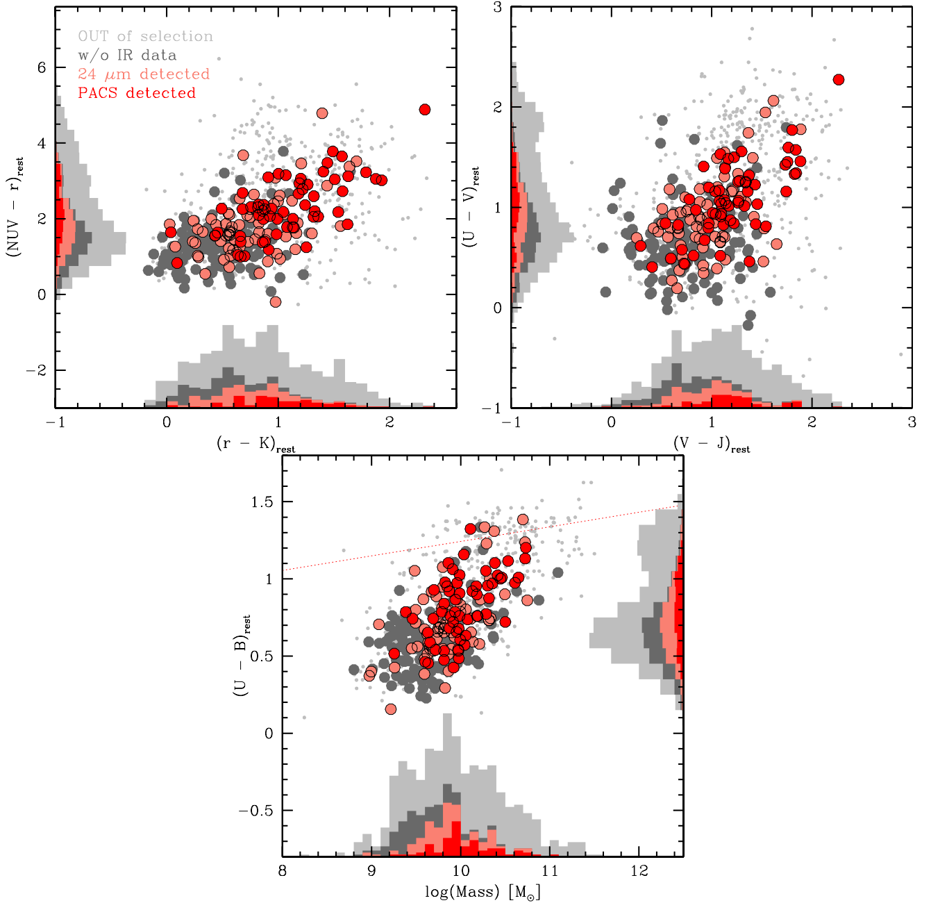
Fig. 6. From top-left, clockwise: a) rest-frame (NUV - r) vs. (r - K) colour diagram (Arnouts et al. 2013); b) rest-frame (U - V) vs. (V - J) colour diagram (Williams et al. 2009); c) rest-frame colour (U - B) vs. stellar mass diagram. The red dotted line is the red sequence at z \sim 2 defined in Cassata et al. (2008). In all plots, small light grey dots represent the GMASS parent sample at z \geq 1 , while large points represent the final sample of 286 SFGs analysed in the paper. In particular: dark grey points indicate galaxies without IR data; salmon points indicate galaxies with a 24 \mu\text{m} detection; red points indicate galaxies with at least one PACS detection. The distribution of each quantity is shown by light grey histograms for the GMASS parent sample (#758), while dark grey histograms represent the distribution over the SFGs sample; salmon histograms represent galaxies with a 24 \mu\text{m} detection; red histograms represent galaxies with at least one PACS detection.
