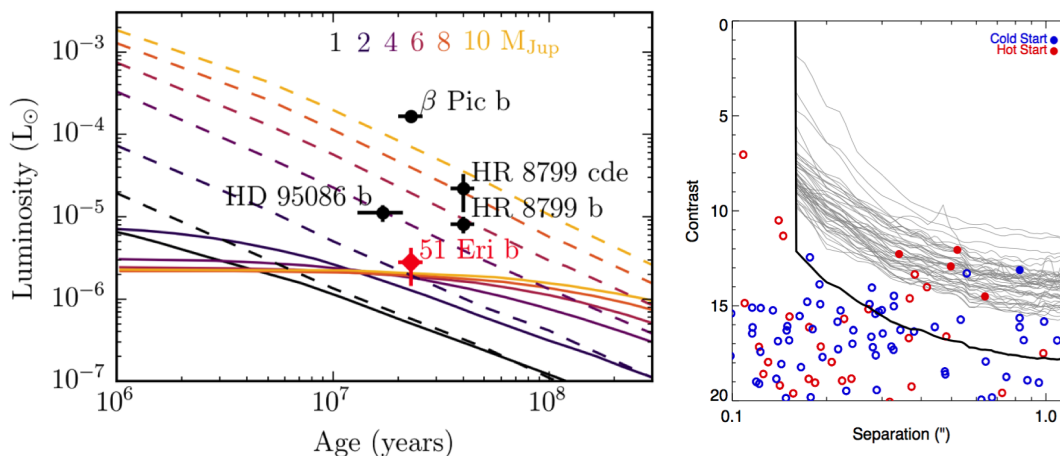
Figure 2: Left: Hot-start (dashed) vs cold-start evolutionary models for 1-10Mj with age vs luminosity. 34 Several known planets indicated. Right: In gray are typical GPI contrast curves with the present instrument. In black is a prediction of improving GPI’s contrast by 3.2 magnitudes. The planet population is modeled using a distribution of planets consistent with radial velocity and direct imaging surveys. Filled circles represent planets that could be detected with the current observations, open circles would fall below the contrast curve for their particular host star.
