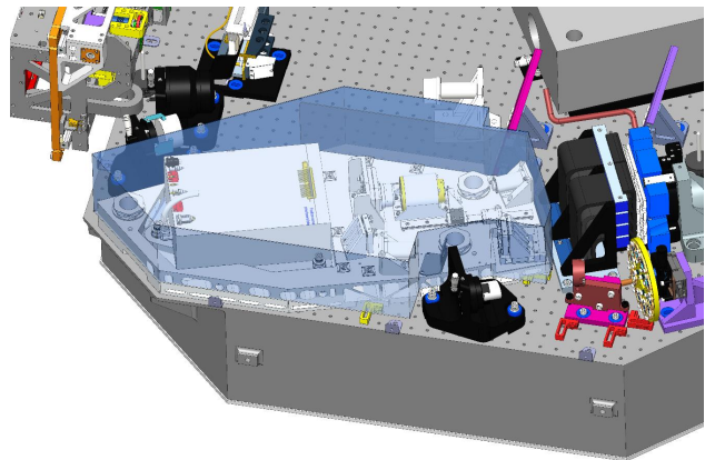
Figure 5: The layout of the upgraded Pyramid based AO bench. 38 Inside of the blue box is the location of the new AO sub-plate, new AO optical components, and PYWFS. Outside of the blue box is the existing GPI optical components which will remain.
