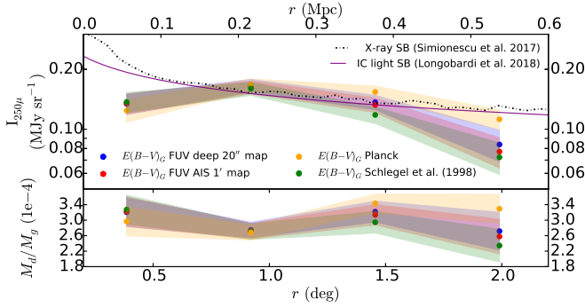
Fig. 3. Radial variation of the Virgo ICD properties (dots). Top panel: expected dust intensities at 250\mu\text{m} as obtained from our E(B - V) measurements. The dash-dotted and full purple lines denote the SB profiles of the X-ray and optical IC light components, respectively. They have been scaled for a direct comparison with the I_{250\mu\text{m}} profile. Bottom panel: dust-to-gas mass ratios. The different colours identify values derived using different Galactic extinction corrections. Shaded areas trace the uncertainties on the mean values that include the standard deviation and the intrinsic measurement errors.
