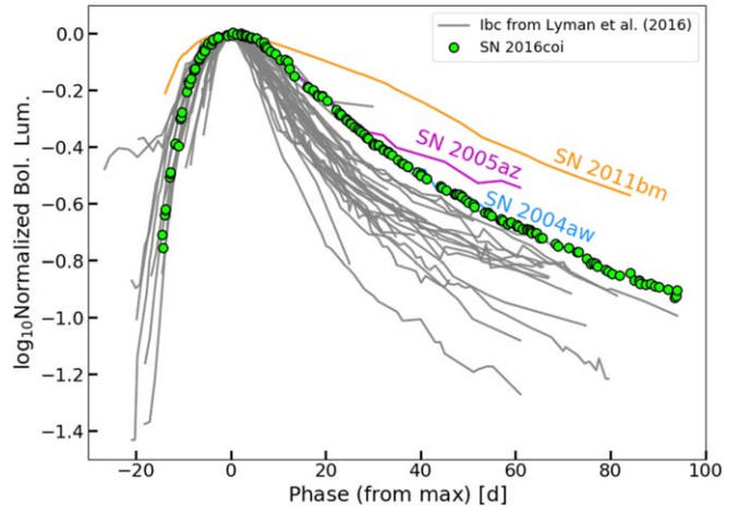
Figure 3. Comparison of the u\text{v}\text{oir} bolometric light curve of SN 2016coi with the sample of SESNe from Lyman et al. (2016). The light curves have been normalized to maximum light. SN 2016coi is among the objects with the broadest light curve, suggesting a larger-than-average diffusion time. The broad light curves of SNe 2004aw (which lies exactly below SN 2016coi; Taubenberger et al. 2006), 2005az (Drout et al. 2011), and 2011bm (Valenti et al. 2012) are also marked.
