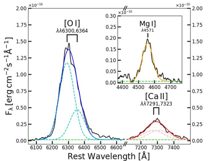
Figure 5. A zoomed-in plot of the spectral region of the [O I] \lambda\lambda 6300, 6364 , [Ca II] \lambda\lambda 7291, 7323 and Mg I] \lambda 4571 lines of the MMT+BlueChannel nebular spectrum acquired on 2017 June 28 ( \sim 400 days after explosion). Gaussian profiles have been used to reconstruct the doublet components of the emission features. The observed lack of asymmetry of the [O I] emission feature might result from spherically symmetric ejecta, or possibly from an axisymmetric explosion, viewed at an angle below 50^\circ .
