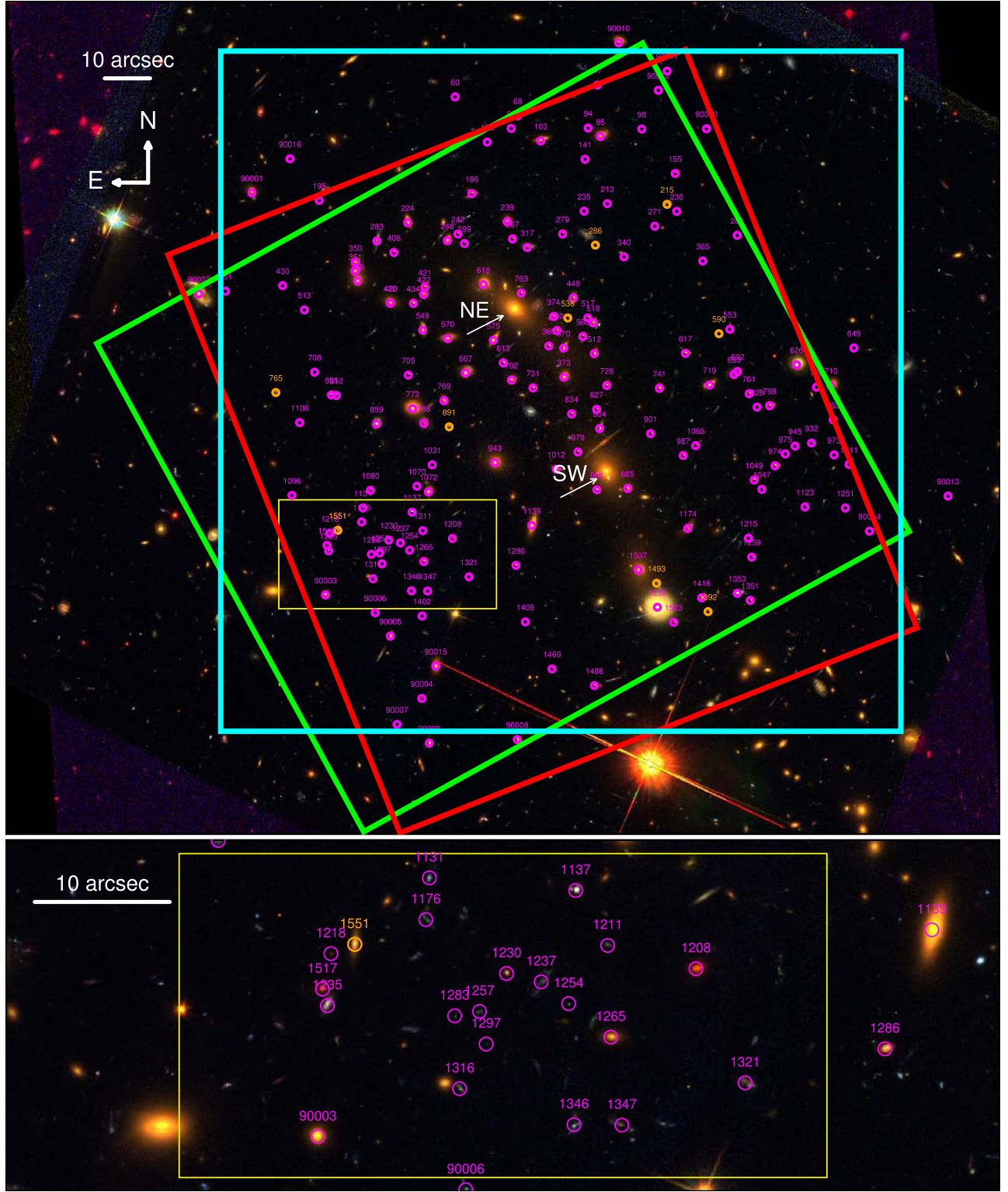
Figure 1. Top panel: all objects that we confirm spectroscopically with GLASS in MACS 0416. The color coding of the circles reflects the quality of the GLASS spectroscopic redshift (see “Quality” in Table 3: 3 = orange, 4 = magenta). The labels on the circles are the GLASS IDs. The two distinct P.A.s of the spectroscopic GLASS pointings are shown by the green (P.A. = 164^\circ ) and red (P.A. = 247^\circ ) squares. There are a few objects that fall outside the direct image field of view (FOV). Their spectra were dispersed onto the chip, so they could still be extracted and analyzed (see Figure 2). The cyan square outlines the area shown in Figure 3. The yellow rectangle shows the zoomed-in region also displayed in the bottom panel. The white arrows point to the two BCGs (NE and SW), which are separated by \Delta V_r \sim 900 \text{ km s}^{-1} (Balestra et al. 2016) and are likely in a merging state (Mann & Ebeling 2012; Jauzac et al. 2015a; Ogrea et al. 2015). Bottom panel: a zoomed-in portion of the field shown in the top panel where the density of confirmed objects is highest. The yellow rectangle is the same one shown in the top panel. In both panels, the color composite image of MACS J0416 is composed of the F435W, F606W, and F814W images from HFF (Lotz et al. 2016) and CLASH (Postman et al. 2012).
