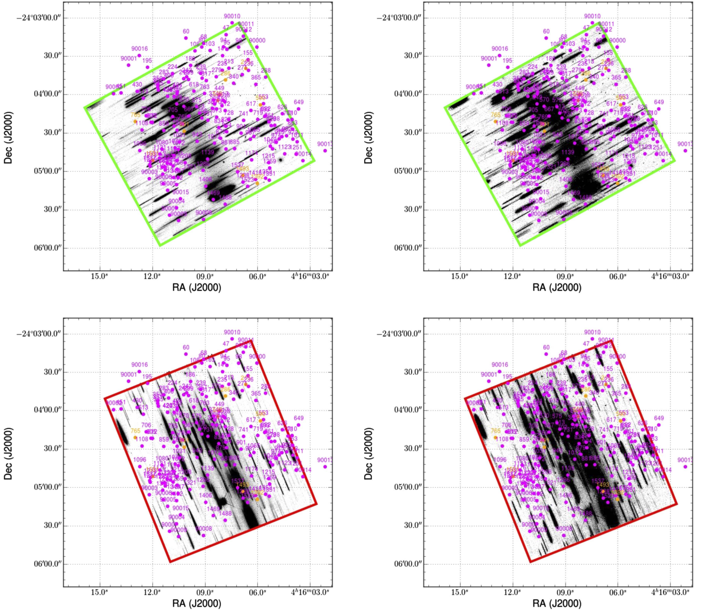
Figure 2. The GLASS G102 (left) and G141 (right) grism pointings of MACS J0416 at two distinct P.A.s, with FOV shown by the green (P.A. = 164^\circ ) and red (P.A. = 247^\circ ) squares. The circles in all panels denote the positions of the emission line objects identified in this work (Table 3), with color coding and labels following the conventions adopted in Figure 1. The circles that fall outside the grism pointings are identified in HST images with a larger FOV than the individual grism FOVs. These objects can still be observed in the grism data because their first-order spectra are dispersed onto the chip.
