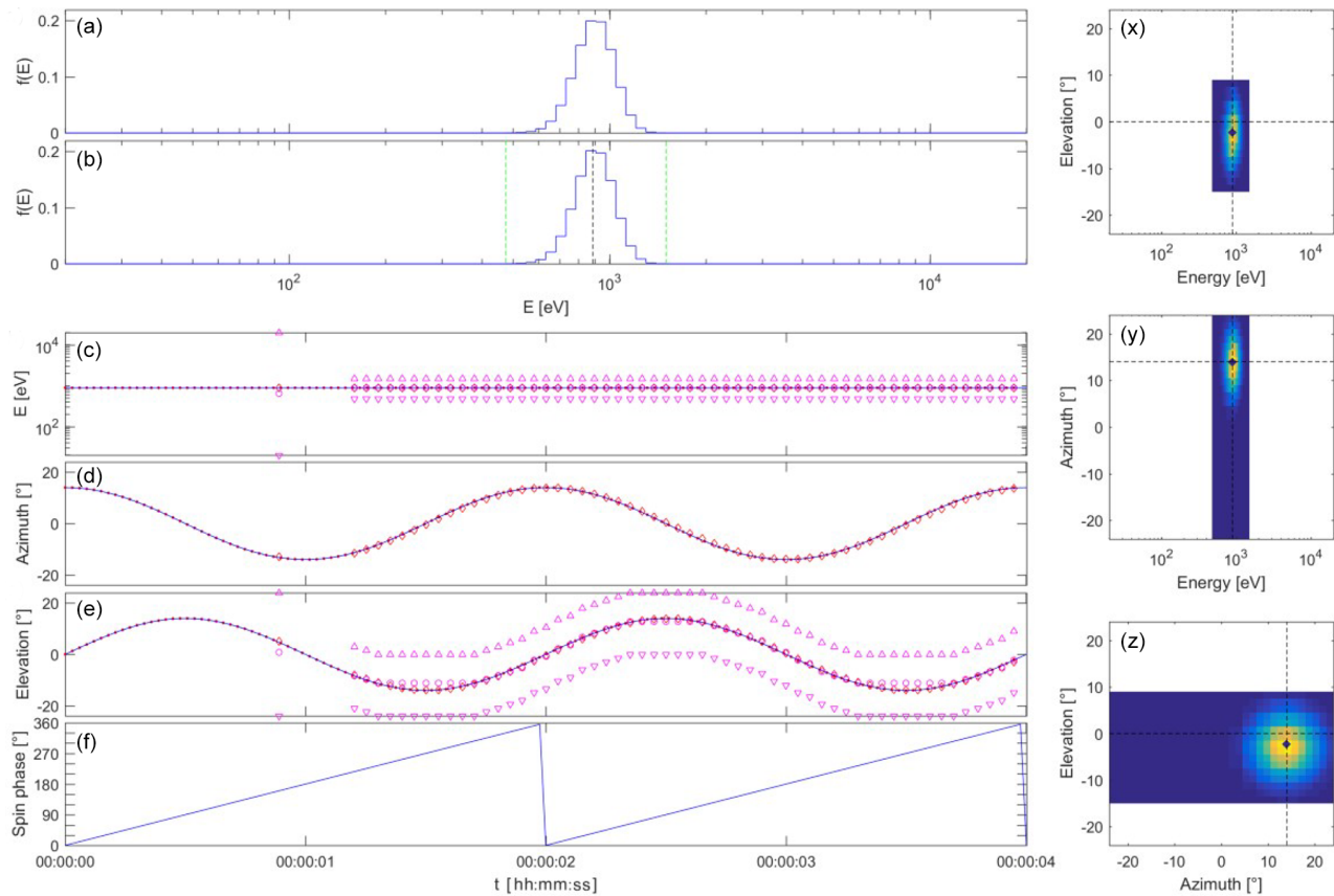
Figure 1. Plasma spectrometer measurements of a constant Maxwellian solar wind beam on a rapidly spinning spacecraft using internal energy and elevation beam tracking. From (a)–(f) and (x)–(z): (a) the energy spectrum of the Maxwellian solar wind; (b) the energy spectrum as acquired by the plasma spectrometer at t = 3.95 s with the vertical black and green dashed lines indicating the centre and the bounds of the sampled energy range; (c) the energy as a function of time, where the horizontal blue line represents the true solar wind value, the small red dots are the Faraday cup measurements every 30 ms (not used with internal beam tracking), the magenta circles and triangles indicate the centre and the bounds of the sampled energy range, and the red diamonds give the mean energy as determined by the plasma spectrometer; (d) the azimuth (same format, no beam tracking for azimuth); (e) the elevation (same format); and (f) the spin phase. The panels at the right hand side show (x) the energy–elevation, (y) energy–azimuth, and (z) azimuth–elevation projections of the VDF at t = 3.95 s. See the main text for more details.
