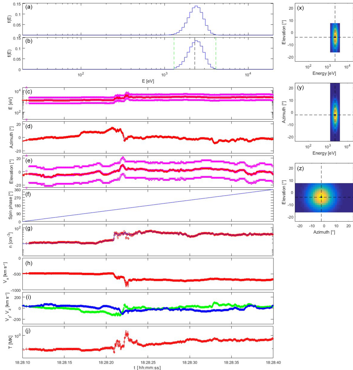
Figure 8. Plasma spectrometer measurements for a solar wind simulation based on Spektr-R/BMSW observations of a strong shock on 22 June 2015, using internal energy and elevation beam tracking. The plot layout is the same as that of Fig. 7.
