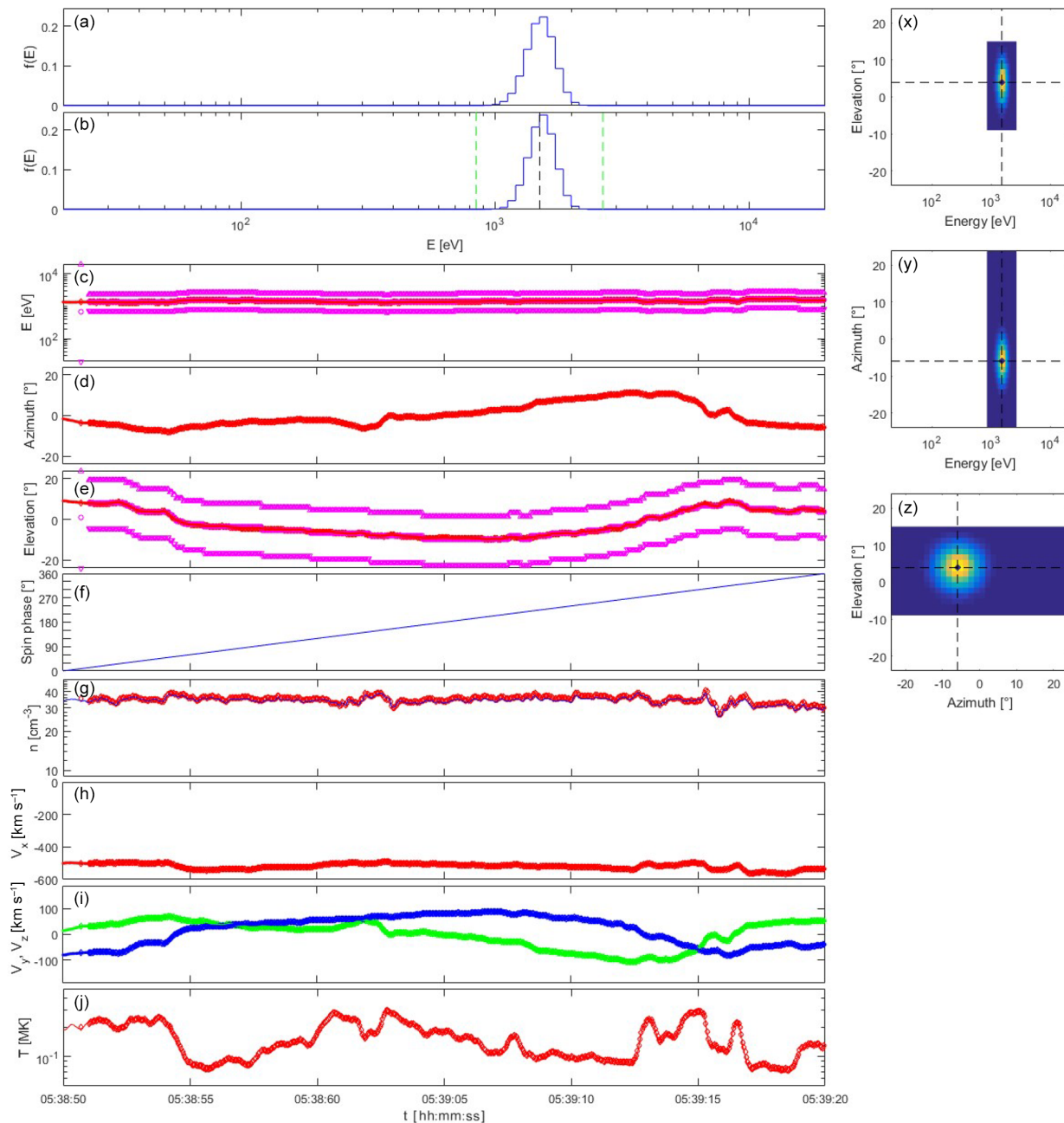
Figure 7. Plasma spectrometer measurements for a solar wind simulation based on Spektr-R/BMSW observations on 8 June 2014, using internal energy and elevation beam tracking. The plot layout is the same as that of Fig. 1, but also shows (g) density, (h, i) velocity in the spacecraft frame of reference ( x axis pointing to the Sun, spacecraft spinning in the x – y plane), and (j) temperature, as a function of time.
