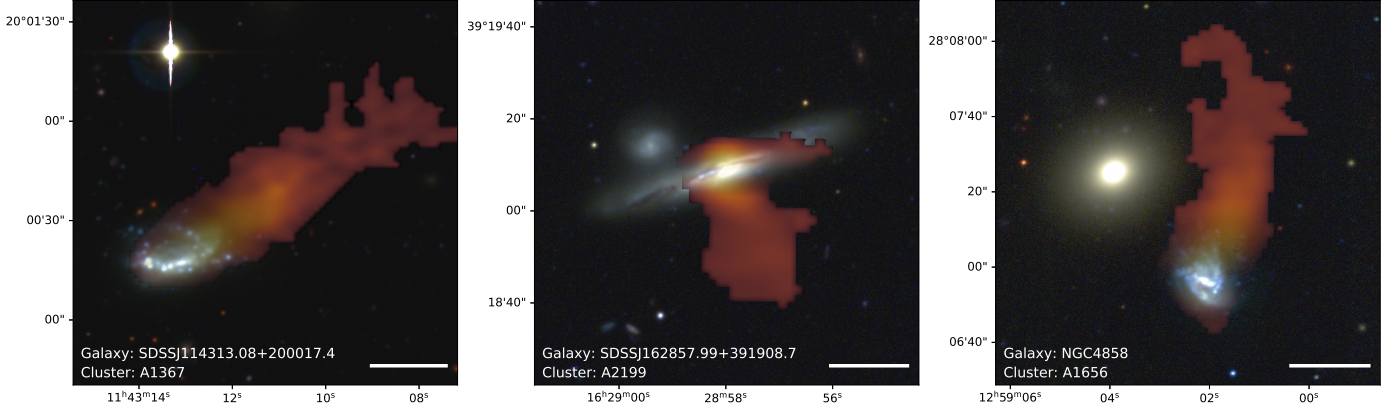
Fig. 2. Composite optical (CFHT, RGB) plus radio (LOFAR, 144 MHz) images of three LoTSS jellyfish galaxies in our sample. The scale bar in each panel corresponds to a physical size of 10 kpc. The radio continuum tail for SDSS J114313.08+200017.4 was first detected at 1.4 GHz by Gavazzi & Jaffe (1985, 1987), the radio continuum tail for SDSS J162857.99+391908.7 is a new detection, and the radio continuum tail for NGC 4858 was first detected at 1.4 GHz by Chen et al. (2020).
