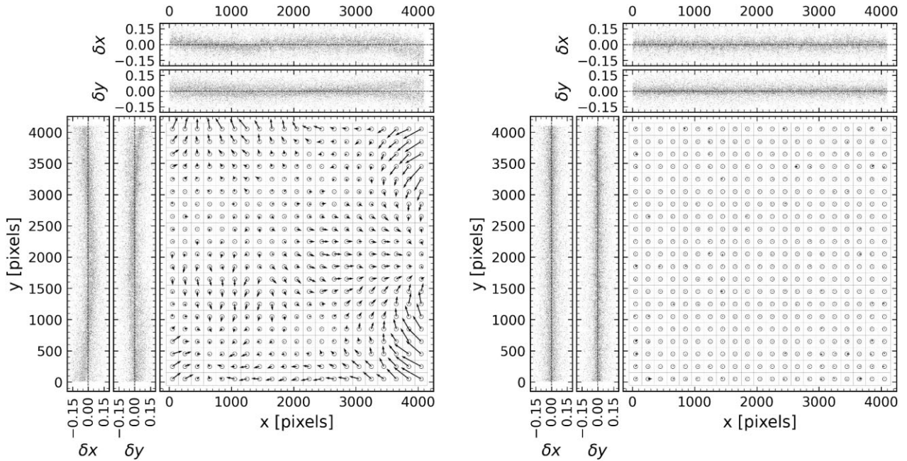
Figure 2. Distortion map for image SC132788 before (left-hand panel) and after (right-hand panel) the distortion correction routine. The central panels represent the CCD coordinate system, with the arrows showing the magnitude and direction of the distortion on each point, corresponding to a 200 \times 200 pixels box. The arrows have been multiplied by a factor 2500 for visualization purposes. On the top and left-hand panels we show a projection on the axes of the x and y components of the distortion.
