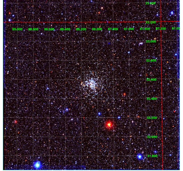
Figure 1. Stacked three-colour image ( u,g,i ) of the field of view, with superimposed a grid with equatorial ICRS coordinates.
