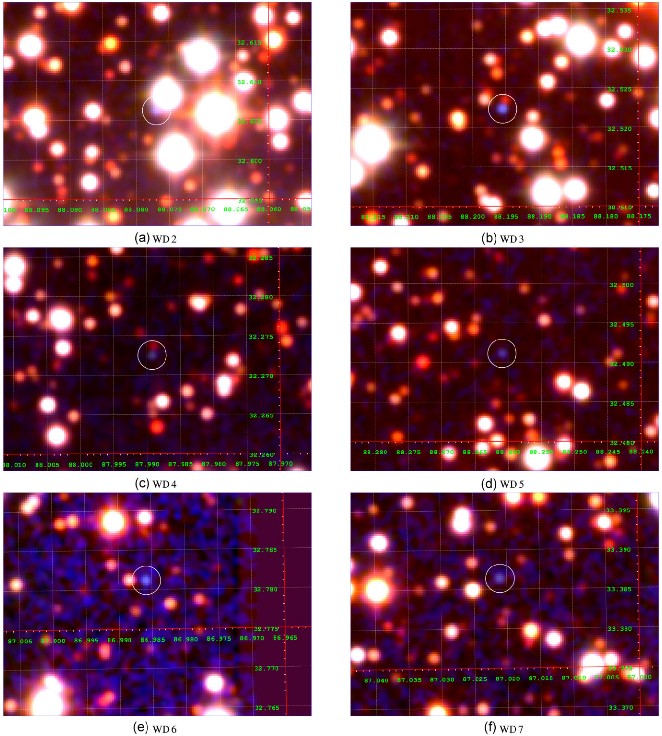
Figure A1. Finding charts of six WD candidates.
