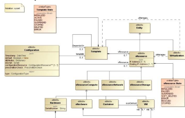
Figure 6: Virtualization data model.
