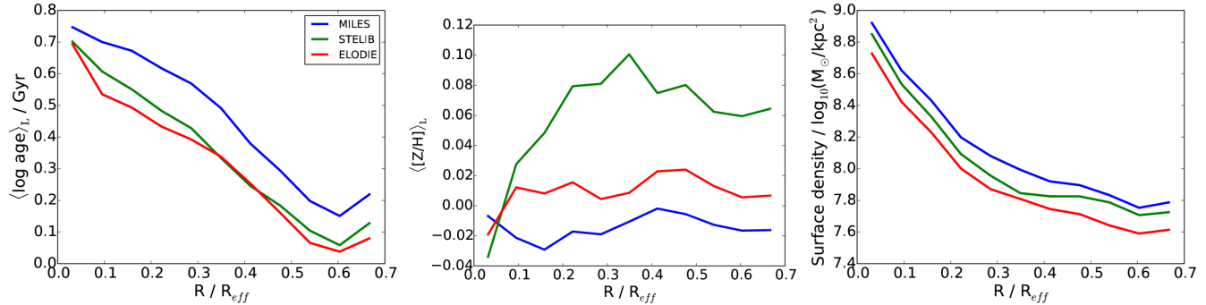
(b) Radial profiles of stellar age, metallicity and surface mass density respectively as a function of stellar library.
