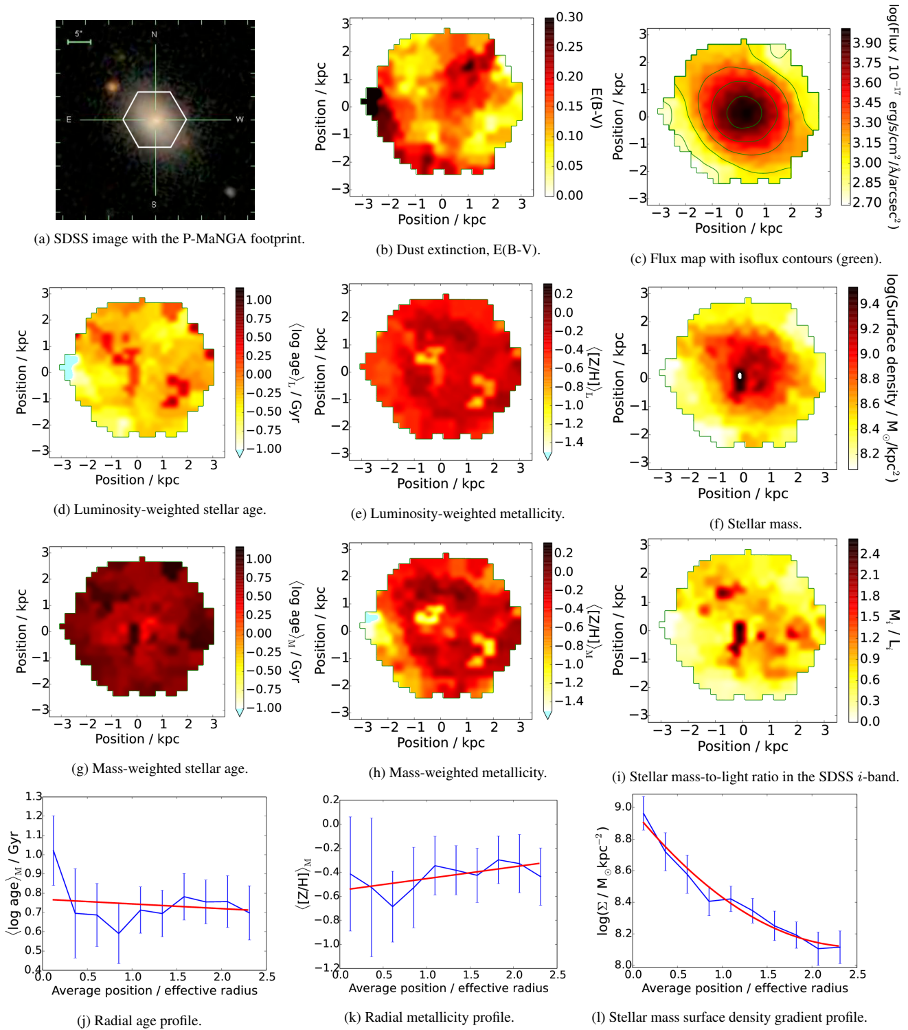
Figure 21. Group \alpha , galaxy p9-19E as in table 2. Stellar population maps and profiles analyzed using MILES-based models with their full parameter range, as described in detail in Figure 5. This galaxy has been observed under good observational conditions with MaNGA-like exposure time and dithering, but covers a larger radial extent than would be targeted in the MaNGA primary sample. However it is selected by the MaNGA secondary sample.
