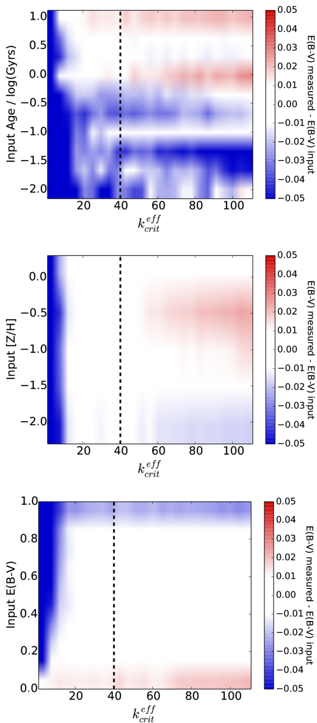
Figure 4. Tests showing the recovery of dust values (in terms of difference between E(B-V) recovered to input E(B-V) ) from mock galaxy spectra from MILES-based models as a function of the number of large-scale modes excluded in the fit. The number of modes excluded is described by an effective k_{crit} parameter (in equation 3). The three plots show recovery of dust as a function of the following input properties: age, metallicity and extinction respectively. In each case, the values plotted are marginalised over the other two input properties. The black dashed line marks the value of k_{crit} used in this paper for the analysis of P-MaNGA galaxies. Each mock galaxy spectra is constructed by perturbing each flux point of an input model SSP by a Gaussian probability distribution on each point, assuming a flat signal to noise of 10 across the whole wavelength range. A signal-to-noise of ten was chosen as it is typical of the outer regions of most P-MaNGA galaxies.
