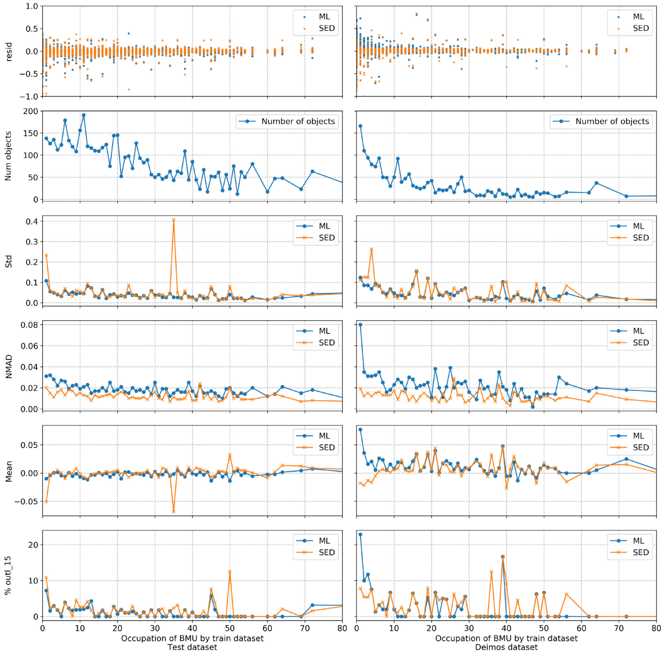
Figure 6. Dependence of the statistics for the test and DEIMOS data sets from the occupation of their BMU by objects from train data set. The x-axis is limited to occupation \leq 80 since there are not enough objects in the cells with bigger occupations to calculate reliable statistics.
