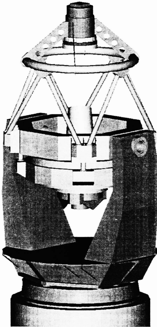
Fig. 5 - A render view of the VST
