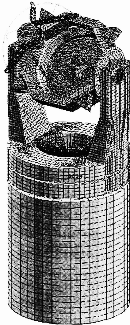
Fig. 6 - Telescope and pillar F.E. model.
