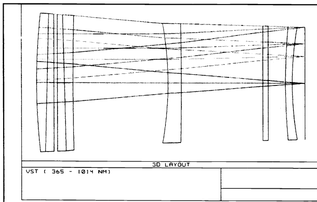
Fig. 1 - Zoom of the optical layout of the VST corrector with the ADC and one lens (B - I bands)
