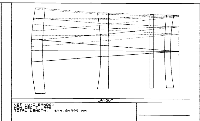
Fig. 2 - Zoom of the optical layout of the VST two-lens corrector (U ÷ I bands)
